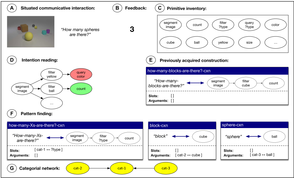
Figure 5 Schematic overview of the acquisition of an item-based construction and two holistic constructions through the processes of intention reading and pattern finding during a situated communicative interaction. An agent observes a question about its environment (A), cannot understand it, and receives the answer to the question as feedback (B). Based on its inventory of primitive operations (C), the agent uses its intention reading capabilities to make a hypothesis about the intended meaning of the observed utterance, which, upon evaluation with respect to the environment, is consistent with the feedback (D). Based on the observed utterance, the meaning hypothesis and a similar yet not identical construction that was previously acquired (E), the agent then applies its pattern finding capabilities to learn an item-based construction and two holistic constructions (F), as well as categorial relations between the constructional slots and their observed fillers (G).
