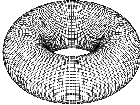
Figure 5: Torus world.
