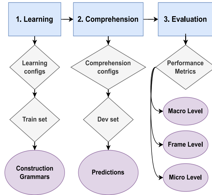
Figure 1: Evaluation Process of the Construction Grammars
