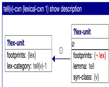
Figure 8: The lexical construction for the verb “tell”. It shows the unit’s designation as a verb ( {v} ) with the lemma “tell” and its category within the grammar as tell(v)-1 . This construction is used to identify and process the verb “tell”.
