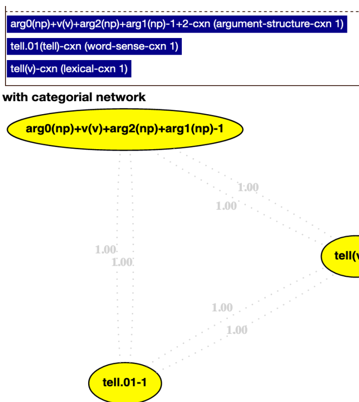
Figure 7: Construction inventory and categorial network after learning “I tell my sister a story”
