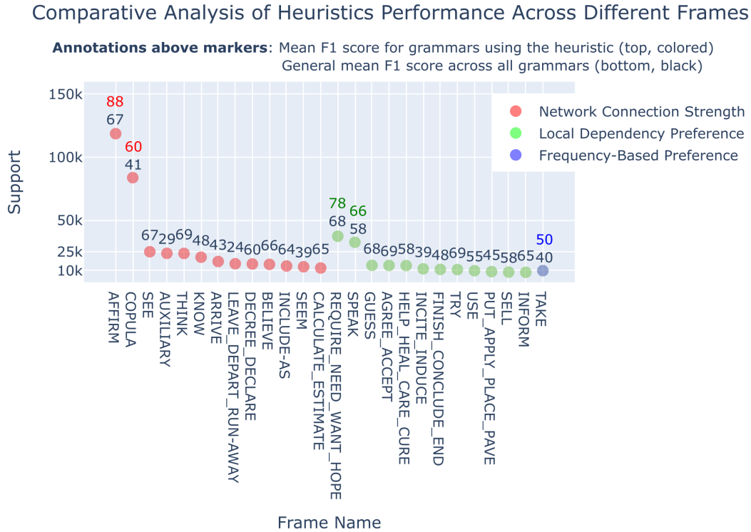
Figure 6: Visualization of heuristics’ performance by frame, highlighting which heuristic achieved the highest F1 score for each frame. Different colors represent distinct heuristics, while the numbers indicate each mean F1 score across all grammars (bottom), and for the highest support frames, an extra number shows the mean F1 score for grammars using the top-performing heuristic (top).
