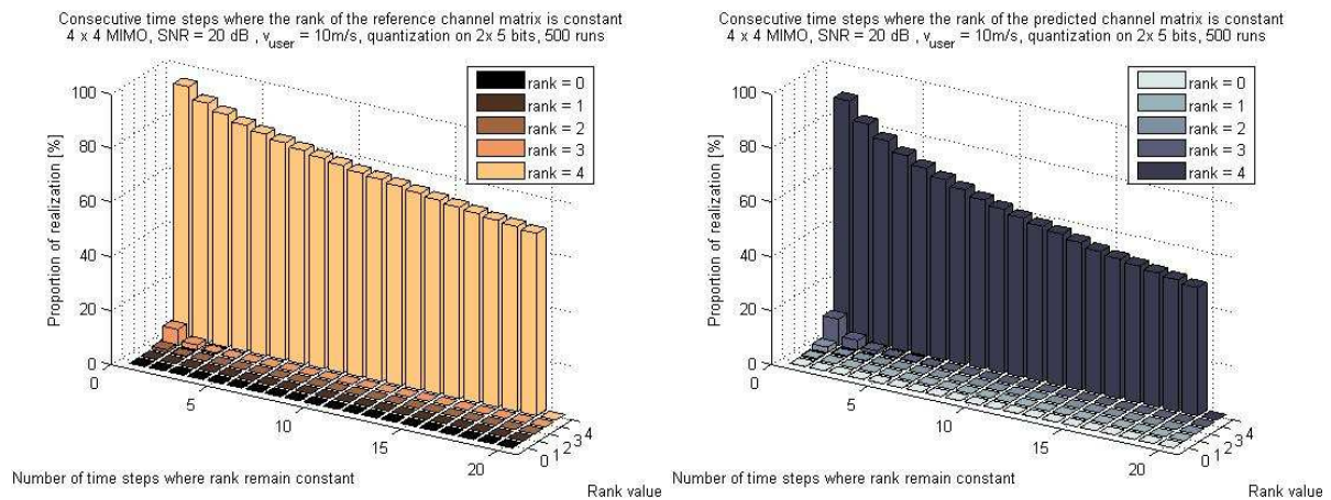
Figure 12-16 : Prediction rank of 4x4 MIMO channel, floating point quantization on 2x 5 bits (SNR = 20 dB)
