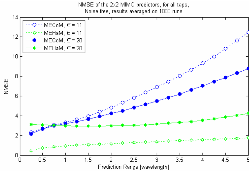
Figure 9-5 : Time evolution of the NMSE of our MIMO predictors in noise free conditions
