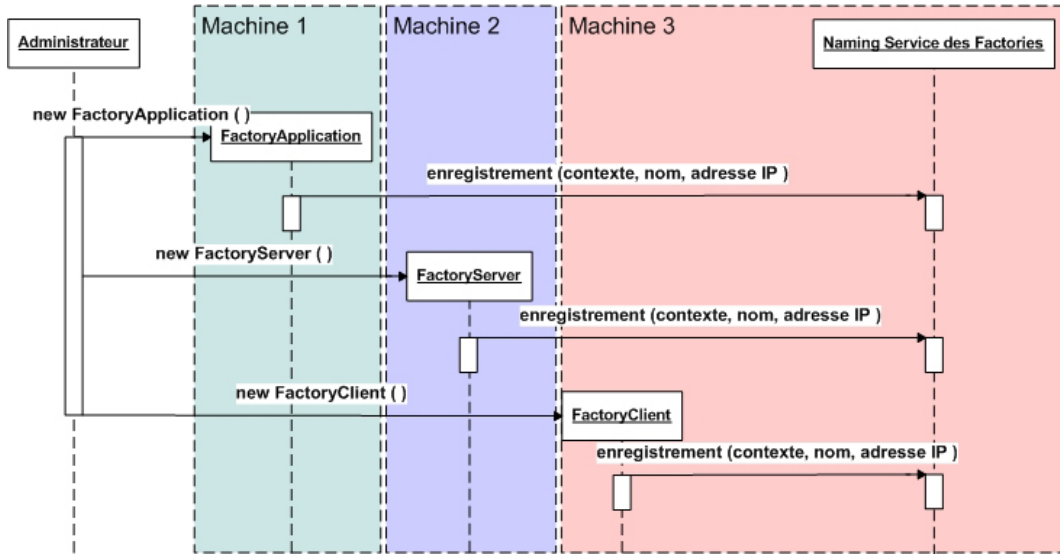
FIG. 3.21 – Lancement des Factories.
