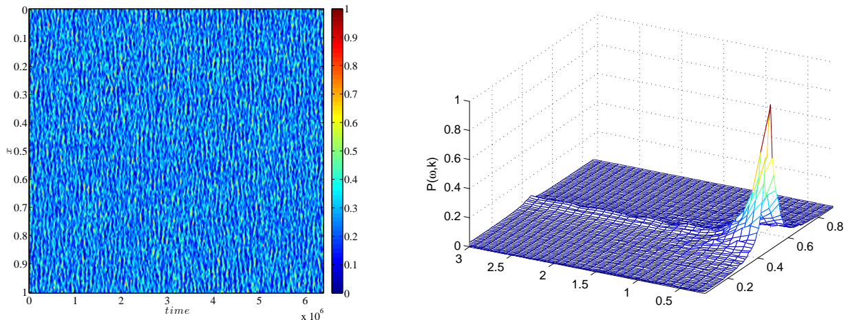
Figure 7: Stochastic patterns for large \mu . Left panel, we report the time evolution of the concentration of A obtained through a numerical integration of 1D system using the Gillespie algorithm with parameters \mu = 0.05 , \zeta = 0.6 , \beta = 1 , \sigma = 1 , \delta = 1/(2\Omega^2) , N = 50 and \Omega = 128 . Right panel, power spectrum in the spatio-temporal domain for the 1D model for the same parameters used in left panel. The numerical power spectrum is obtained by averaging over 150 independent realisations.
