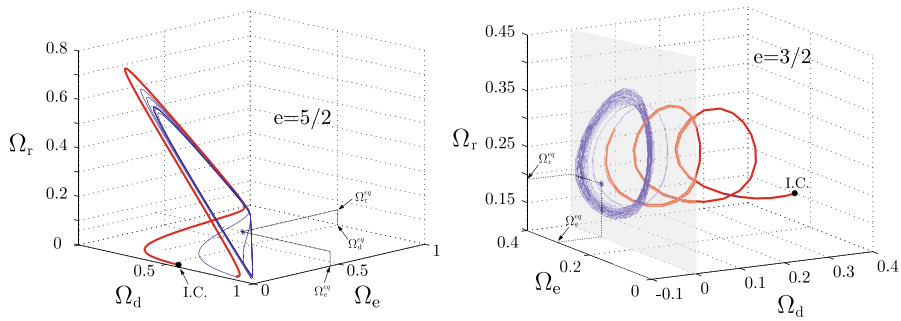
Fig. 3 Evolution of the three coupled density parameters, in the 3D phase space. The beginning of the orbit is overlined. Initial condition is indicated by a black dot . Relevant equilibria are indicated by a star
