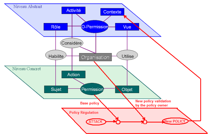
Figure 5: Policy regulation in the Or-BAC model. In the Figure 5, we mainly added a layer (the bottom layer) in order to illustrate the proposed regulation process of section IV.
