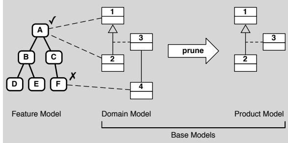
Figure 1. Pruning of a large model
