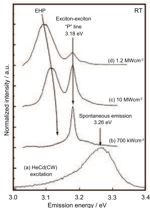
Fig.22 Normalized PL spectra of ZnO epitaxial layers for various excitation intensities at room temperature [44]
