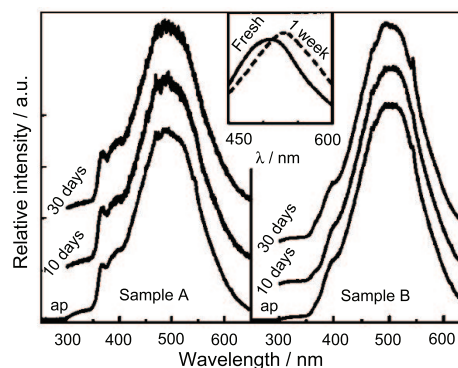
Fig.16 Dependence of PL spectra of samples A and B on aged period: as-prepared powders (ap), aged over 10 d, and aged over 30 d. Inset is the PL spectra of the ZnO colloid (0.1 mol/L); solid line: fresh colloid and dashed line: 1 week aged colloid [138]
