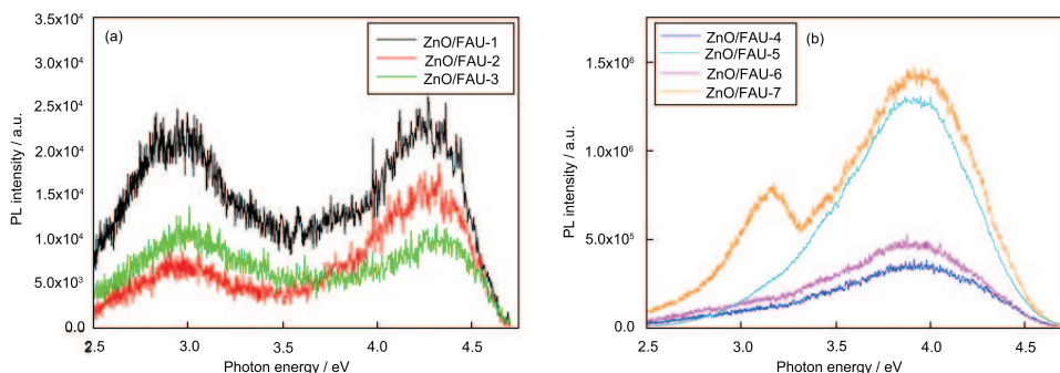
Fig.28 PL spectra of the ZnO/FAU nanocomposites with low ZnO loadings (a) and high ZnO loadings (b) ( E_{exc}=6.4 eV) [176]
