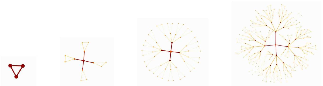
FIG. 3: The “Cantor dust” WFN, s = 4 , f = 1/5 and G_0 is a triangle. From the left to the right G_0 , G_1 , G_2 and G_3 . Gray scale (color on-line) reproduces edges weights: the darker the color the larger the weight. The dimension of the fractal is \log 4 / \log 5 \sim 0.8614 . Visualization was done using Himmeli software [16].
