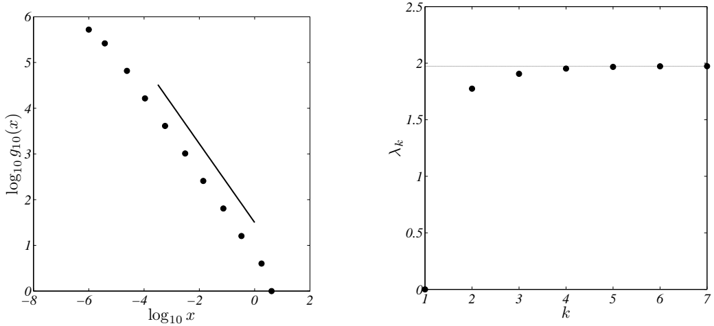
FIG. 5: The “Cantor dust” WFN, s = 4 , f = 1/5 and G_0 is made by a triangle. Left panel, node strength distribution for G_{10} composed by 873813 nodes; the reference line has slope -\log 4/\log 5 \sim -0.861 , a linear best fit (data not shown) provides a slope -0.865 \pm 0.015 and R^2 = 0.9998 . Right panel, average weighted shortest path for G_k , k \in \{1, \dots, 7\} . The horizontal line represents the asymptotic value predicted by (9).
