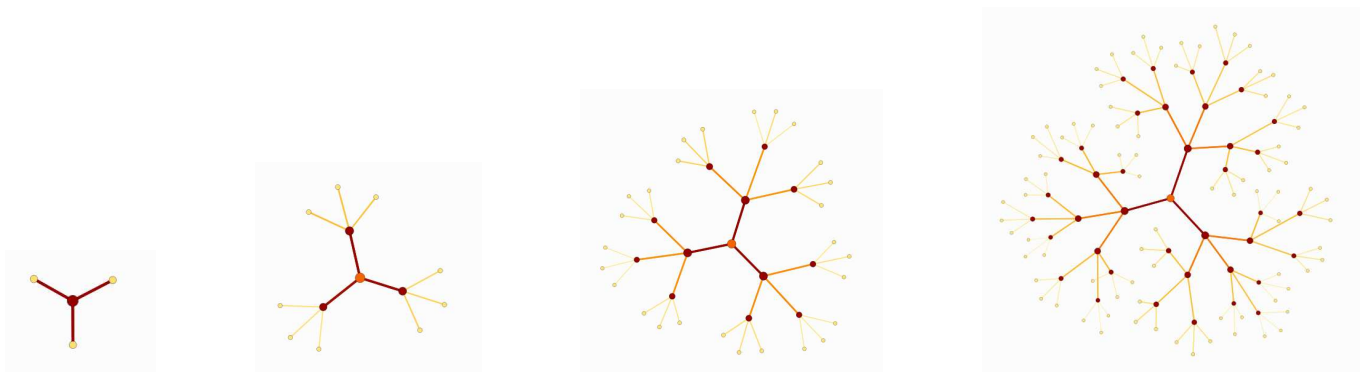
FIG. 2: The “Sierpinski” WFN, s = 3 , f = 1/2 and G_0 is composed by a single node. From the left to the right G_1 , G_2 , G_3 and G_4 . Gray scale (color on-line) reproduces edges weights: the darker the color the larger the weight. The dimension of the fractal is \log 3 / \log 2 \sim 1.5850 . Visualization was done using Himmeli software [16].
