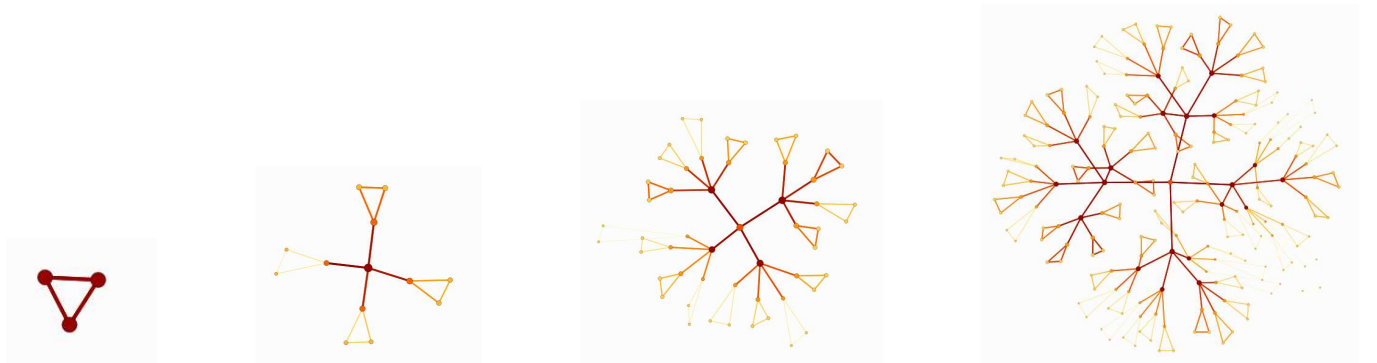
FIG. 7: The non-homogeneous “Cantor dust” WFN, s = 4 , f_1 = 1/2 , f_2 = 1/3 , f_3 = 1/5 , f_4 = 1/7 and G_0 is formed by a triangle. From the left to the right G_0 , G_1 , G_2 and G_3 . Gray scale (color on-line) reproduces edges weights: the darker the color the larger the weight. Visualization was done using Himmeli software [16].
