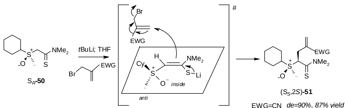
Scheme 19
