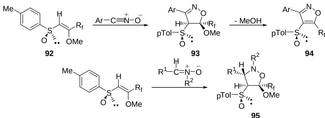
Scheme 36
