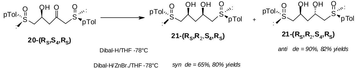
Scheme 5
