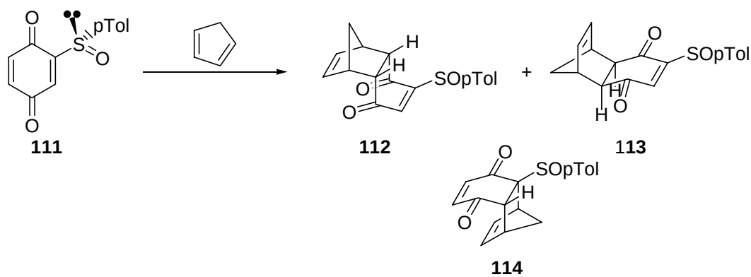
Scheme 42
