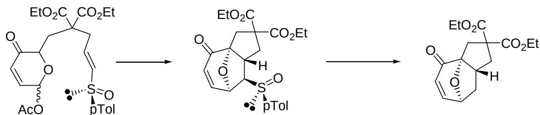
Scheme 65
