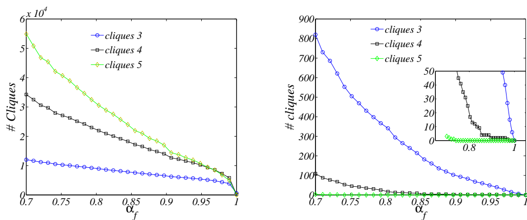
Fig. 5. Number of maximal 3, 4 and 5-cliques in the social network once consensus has been achieved. Parameters are N = 100 , \Delta O_c = 0.5 , \alpha_c = 0.5 . Right panel, \sigma = 0.5 , the network exhibits the weak ties property. Left panel, \sigma = 0.1 , the network does not display the weak ties phenomenon.
