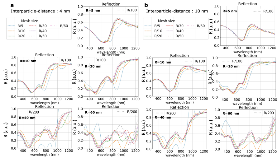
Fig. 5. Reflection spectra for all mesh sizes and all radii for an interparticle-distance of 4 nm (a) and 10 nm (b).
