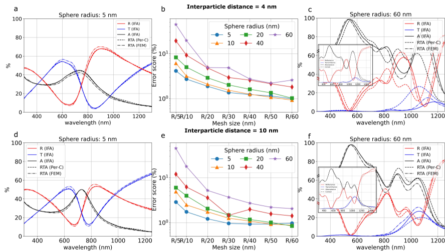
Fig. 7. RTA spectra simulated by FDTD with IFA (solid lines) and Per-C (dashed lines) meshes and by FEM (dash-dotted lines). Spectra (a) and (c) were computed with spheres of 5, 60 nm, respectively, at an interparticle distance of 4 nm. Spectra (d) and (f) were computed with spheres of 5, 60 nm, respectively, at an interparticle distance of 10 nm. The FDTD spectra were simulated with a mesh size of R/60. Figures (b) and (e) show the error scores for the IFA FDTD simulations with the FEM simulations taken as reference. Inserts in Figures (c) and (f) are computed with a R/100 mesh size.
