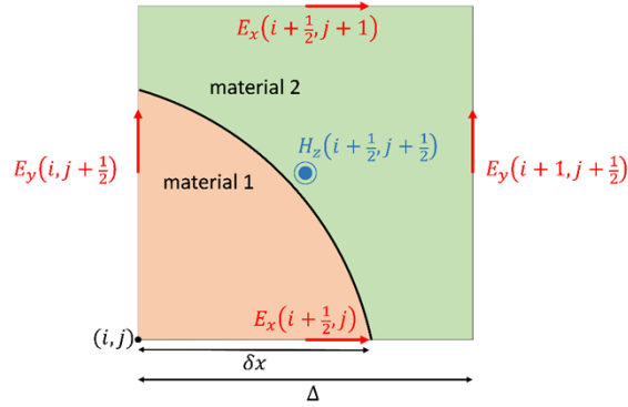
Fig. 2. 2D representation of the interface field averaging method. The indices “ i ” and “ j ” are taken along the two perpendicular periodic directions. \Delta is the mesh size, i.e., the size of Yee-cell in the x direction.
