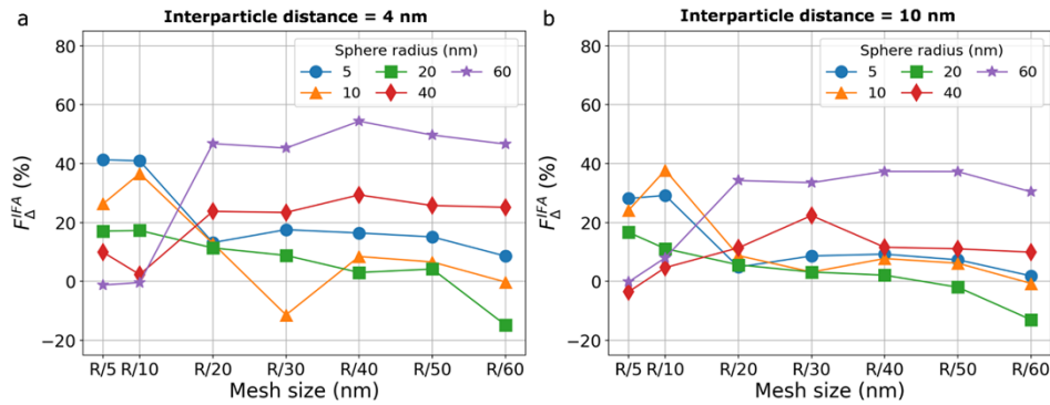
Fig. 6. Impact of the IFA on the convergence for an interparticle distance of 4 nm (a) and 10 nm (b). Positive values of F_{\Delta}^{IFA} signify that IFA improves the convergence with respect to Per-C meshing.
