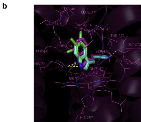
Fig. 7. (a, top), Sequence alignment used for modeling of hTDO: residues of catalytic site area (4 Å, underlined), conserved residue (pink), similar residues (yellow) and different residues (blue) and (b, bottom) docked structure of (1) (blue), (2) (green) and (3) (pink) into the active site of rmTDO.
