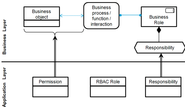
Figure 8. Permission-responsibility assignment optimization.
