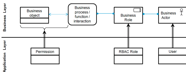
Figure 3. User-role and permission-role assignment.
