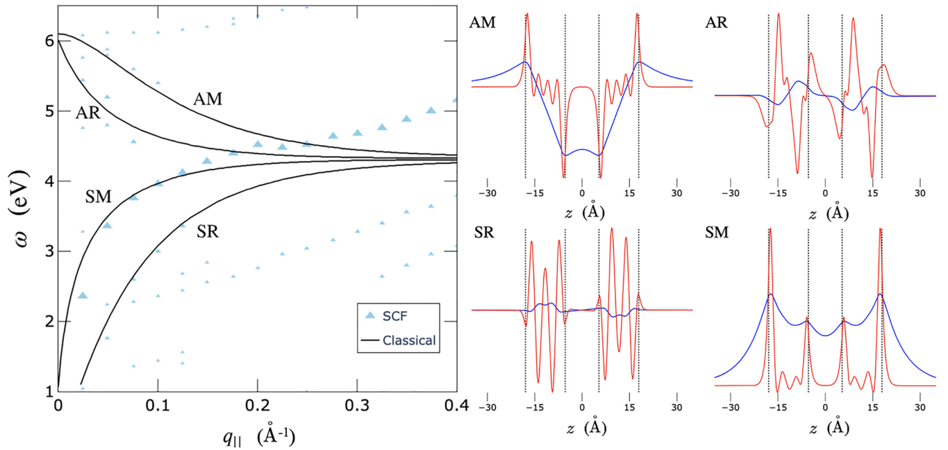
FIG. 6. Dispersion relation of the double symmetric six-atomic layer Na equivalent slab system with a gap of 9.82 Å using the surface response function (SRF). Left: In black, the prediction of the classical theory from Eqs. (38) and (39). In blue, the prediction from the self-consistent field (SCF). The size of the dots is proportional to the intensity of the mode (relative intensity for each q_{||} ). Right: The four modes associated with each branch with the typical shape of the variation of, in red, the density \rho_i(z) and, in blue, of the potential V_i(z) associated with the mode. Top left is the antisymmetric mirrored (AM) mode, top right is the antisymmetric reversed (AR) mode, bottom left is the symmetric reversed (SR) mode, and bottom right is the symmetric mirrored (SM) mode. q_{||} = 0.1 \text{ \AA}^{-1} for the SR, SM, and AM modes, and q_{||} = 0.75 \text{ \AA}^{-1} for the AR mode.
