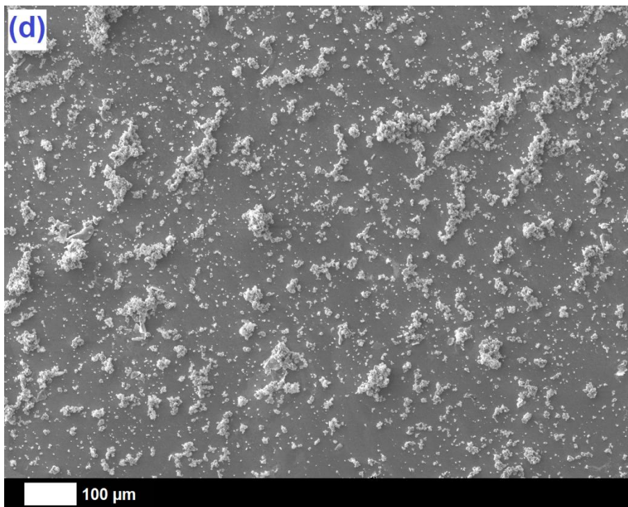
Fig. 9. SEM pictures of hydroxyapatite deposited on Ti substrates covered by (a) pristine Ta 2 O 5 and composite (b) Ta 2 O 5 /O-MWCNTs, (c) Ta 2 O 5 / weak P-MWCNTs, and (d) Ta 2 O 5 / strong P-MWCNTs coatings.
