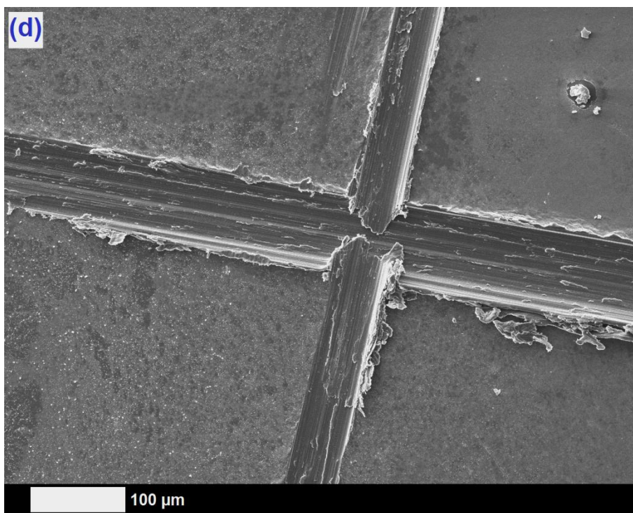
Fig. 6. SEM pictures after peeling tests of Ti substrates covered by (a) pristine Ta 2 O 5 and composite (b) Ta 2 O 5 /O-MWCNTs, (c) Ta 2 O 5 / weak P-MWCNTs, and (d) Ta 2 O 5 / strong P-MWCNTs coatings.
