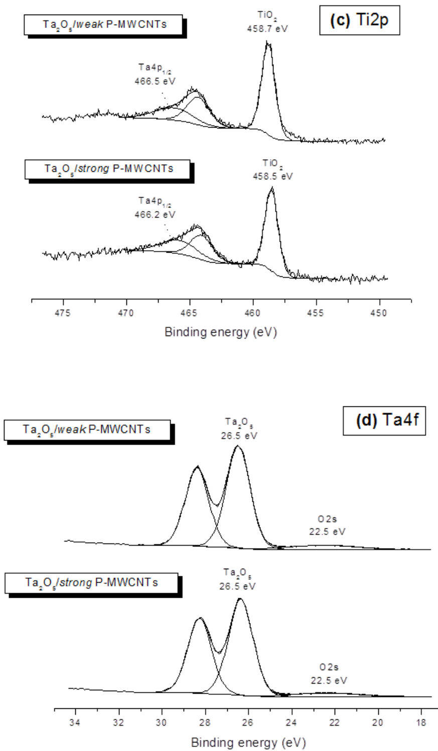
Fig. 4. XPS survey spectra (a) and core levels of C1s (b), Ti2p (c) and Ta4f (d) of composite coatings of Ta_2O_5 and weak P-MWCNTs (up) and strong P-MWCNTs (down) generated on Ti.
