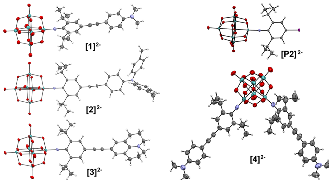
Figure 2. ORTEP representations of the complex anions in [NBu 4 ] 2 [P2] and [NBu 4 ] 2 [1] to [NBu 4 ] 2 [4]. Thermal ellipsoids are drawn at the 30% probability level. Disorder in the julolidinyl group of [3] 2- has been omitted for clarity but is shown in Figure S12 (Supporting Information). Color scheme: C is gray; N, purple; O, red; Mo, green; I, purple. H atoms are represented by white spheres of arbitrary radii.
