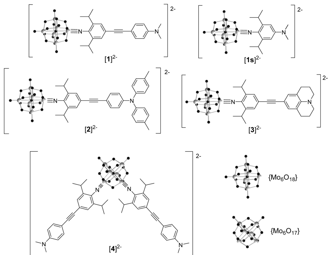
Figure 1. Structures of complex anions [1] 2- to [4] 2- synthesized for this study and previously published 11 [1s] 2- included for comparison. All compounds were isolated as tetrabutylammonium salts.
