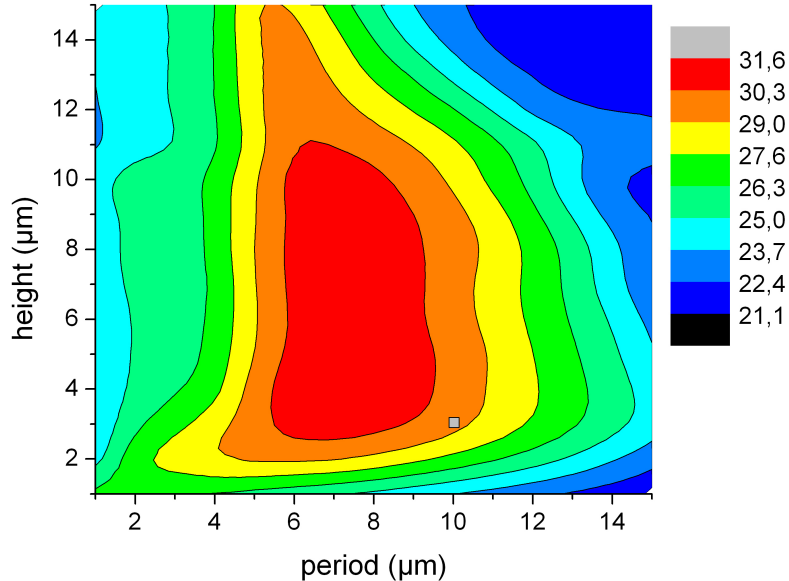
FIG. 4: Optimal geometry for the tilted scale (or the so-called firefly) geometry. The map shows the light extraction percentage as a function of the period and the height. The grey rectangle shows the geometry of the firefly.
