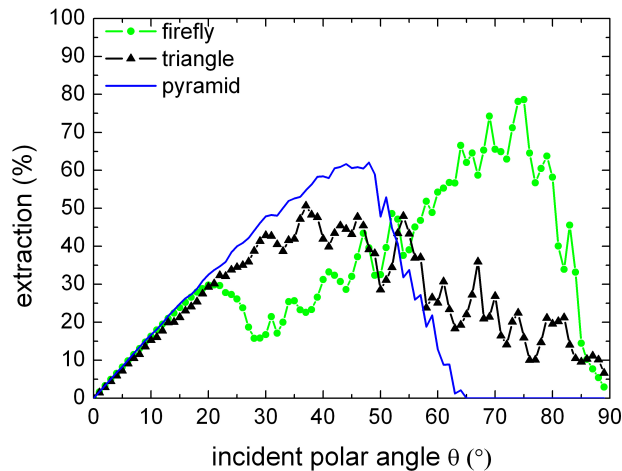
FIG. 9: Comparison between the light extraction in the best geometry and the most effective direction for the different structures. The firefly extracts the light in the most efficient way.
