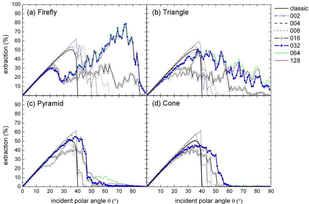
FIG. 6: Convergence calculation for the different structures. The incident azimuthal angle has been fixed to \phi = 90^\circ . The incident polar angle varies from 0^\circ to 90^\circ . 32 plane waves are enough to show properly the effect of the different structures.
