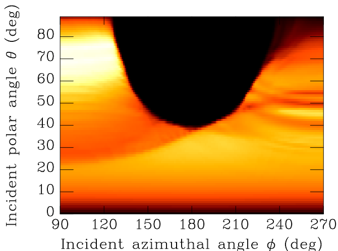
FIG. 3: Map of the relative extraction intensity in function of the incident polar angle and the incident azimuthal angle. The light is highly extracted when the lightrays are impinging on the surface perpendicular to the edge of the protruding structure and perpendicular to the slope. The color scale is relative: black shows zero transmission, and white shows maximal transmission.
