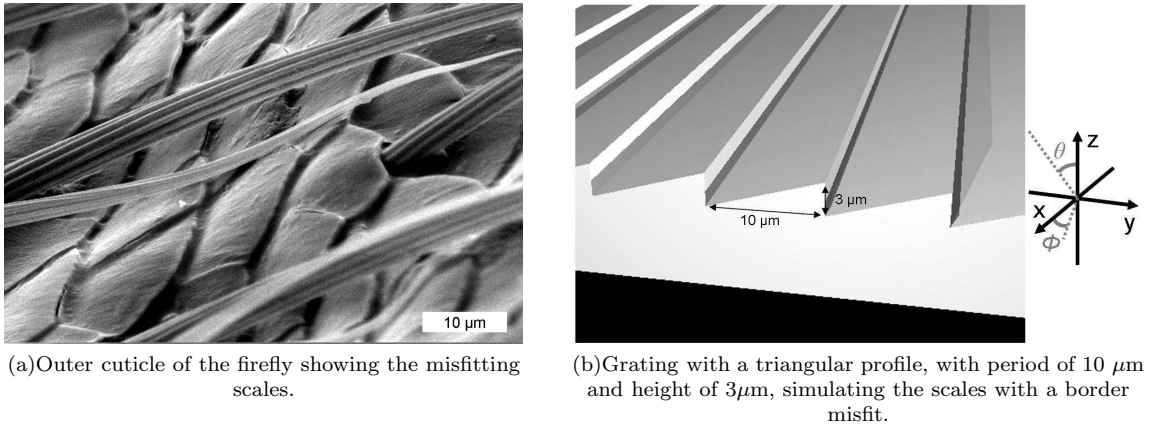
FIG. 1: Structure found on the outer surface of the firefly-cuticle
