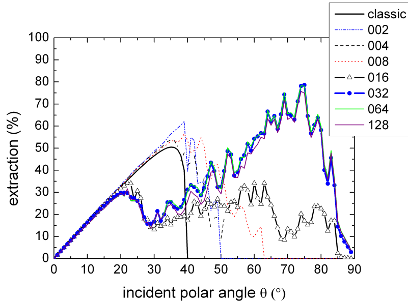
FIG. 2: Convergence study of the tilted scales. The incident azimuthal angle has been fixed perpendicular to the tilted edges ( \phi = 90^\circ ). The incident polar angle varies from 0^\circ to 90^\circ . 32 plane waves are enough to show properly the effect of the tilted scales. The critical angle is lost and a huge part of the light is extracted at high incident polar angles.
