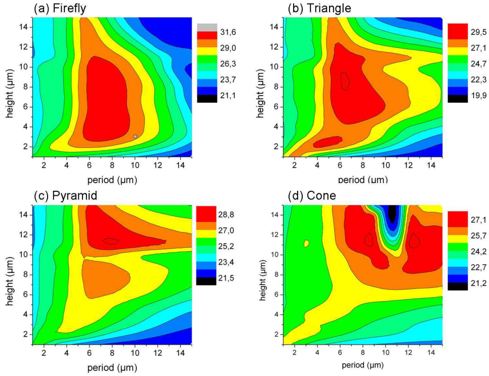
FIG. 7: Optimal geometry for the different structures. Maps showing the light extraction percentage as a function of the period and the height.
