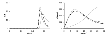
Fig. 8 Distance and angle distributions of Ubiquitin-water H-bonds.
