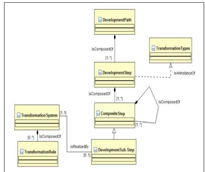
Figure 1: Transformation path, step and sub-step [8]
