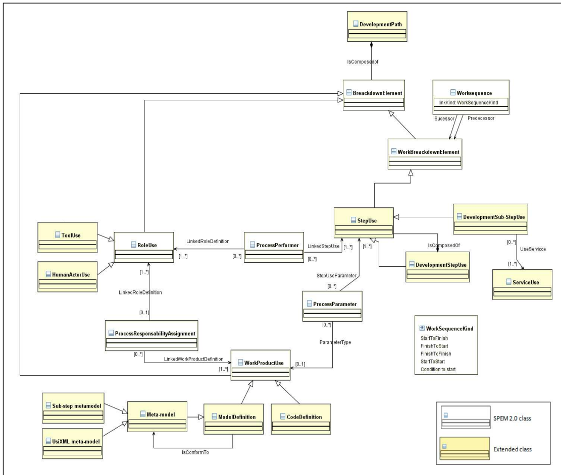
Figure 4: SPEM4UsiXML Process Structure package
