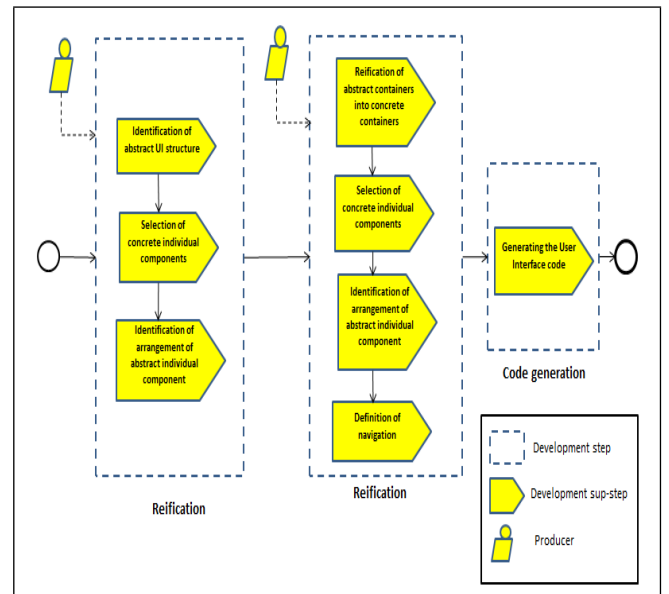
Figure 5: UsiXML Forward Engineering method expressed in SPEM4UsiXML
