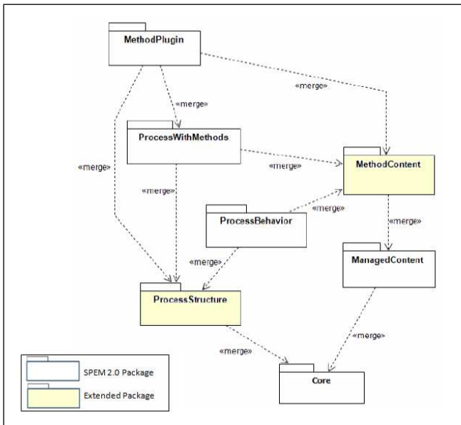
Figure 3: Structure of the SPEM4UsiXML meta-model
