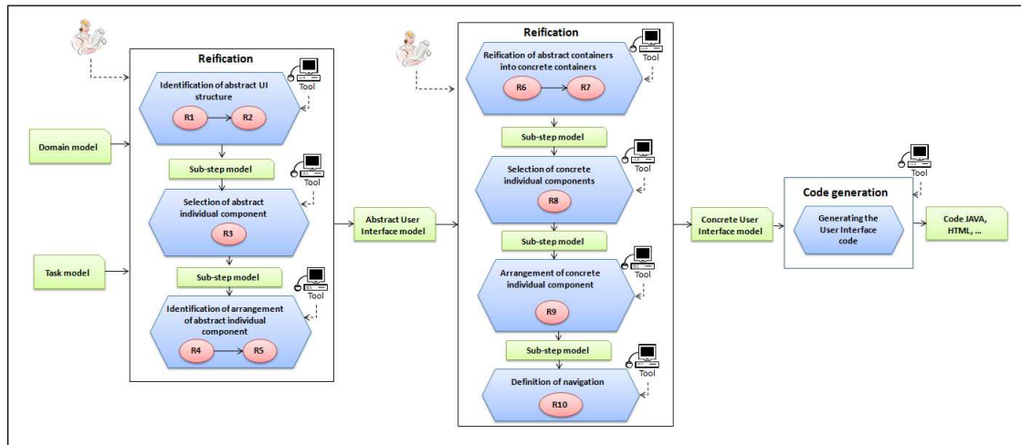
Figure 2: Forward Transformational Development of UIs
