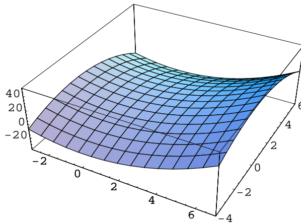
Figure 1: Surface defined by z = x^2 - y^2 for -3 < x < 7 and -4 < y < 6
