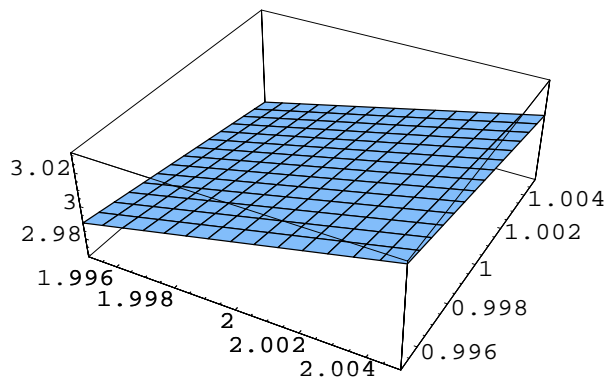
Figure 2: Surface defined by z = x^2 - y^2 for 1.995 < x < 2.005 and 0.995 < y < 1.005
