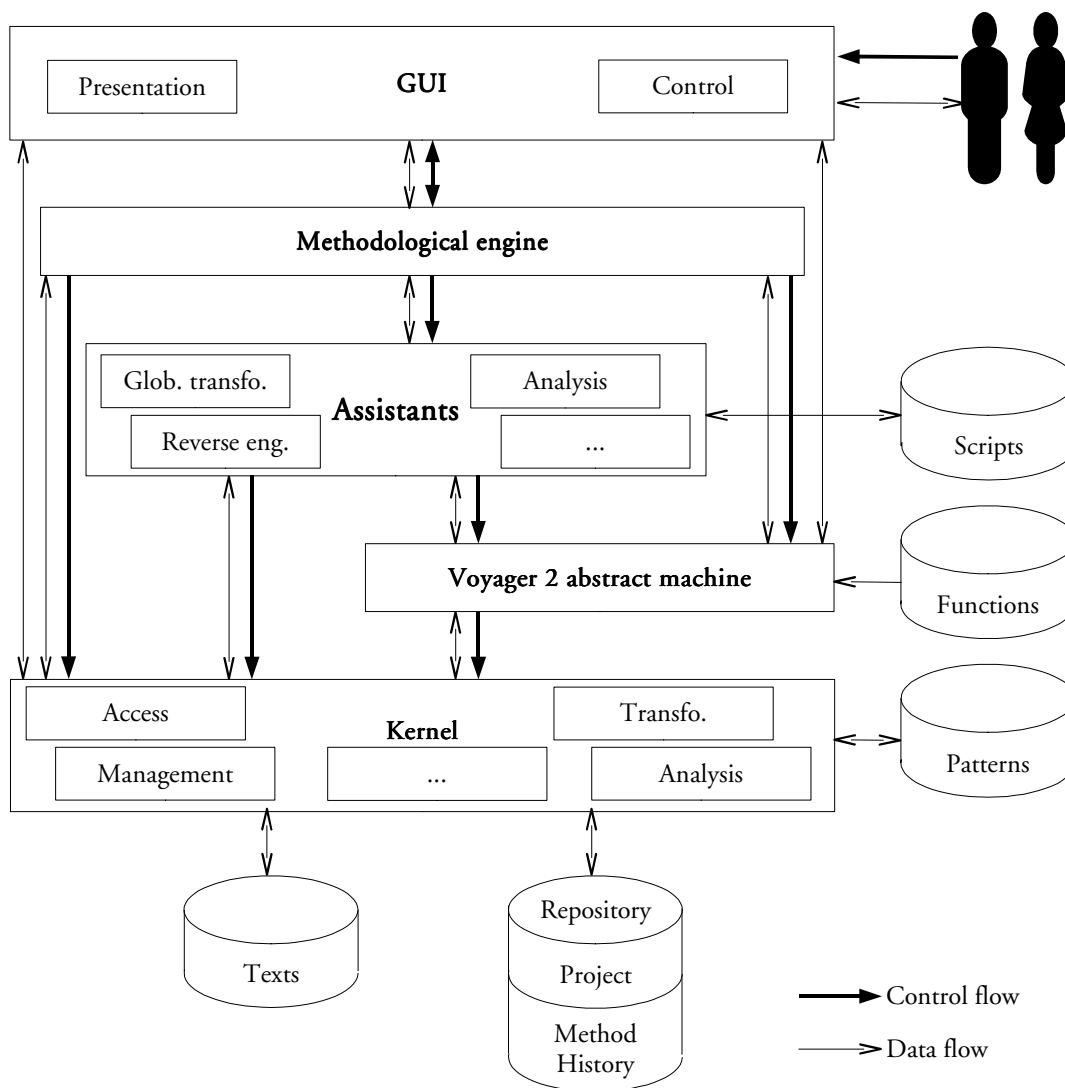
Figure 10.1 The general DB-MAIN architecture
