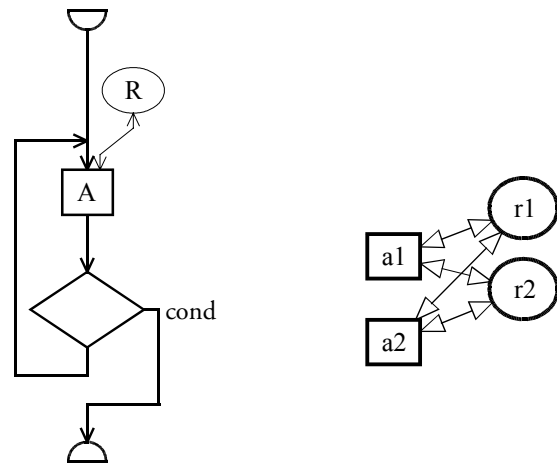
Figure 4.9 A standard repeat...until loop
