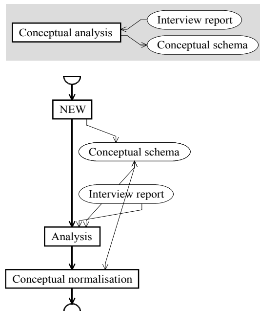
Figure 11.2 Conceptual analysis strategy
