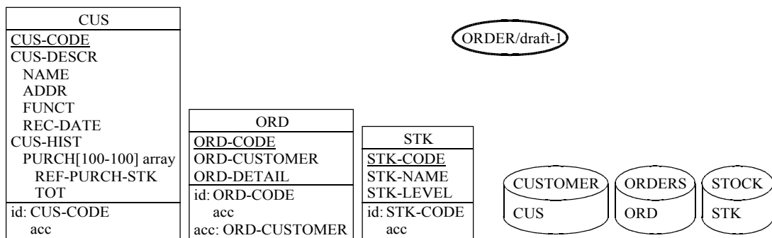
Figure 11.30 The long fields of record CUS are refined
