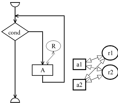
Figure 4.8 A standard while loop
