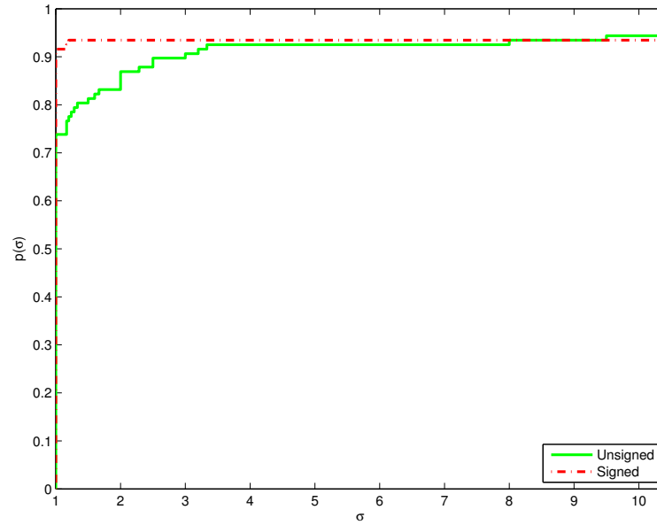
Figure 8.15: Filter size performance profile for the filter variants using unsigned and signed filter entries
