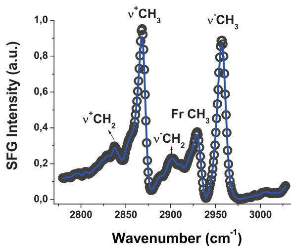
Figure 7.13: SFG spectrum of 100 \mu\text{m} DDT stripes backfilled with mercapto-dodecanol. The resemblance with the one of the lone DDT printed stripes (chapter 6) attests that the backfilling step does not damage the printed DDT layer and leads simultaneously to a fairly organized mercapto-dodecanol film since only weak methylene activity is detected.
