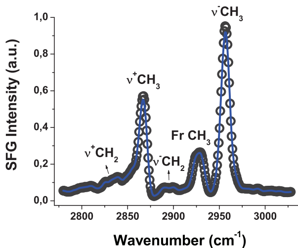
Figure 7.11: SFG spectrum of supported DNP lipid layer. The sample is realized by transferring the film from the trough (Langmuir-Schaefer) to the solid substrate by means of a stamp (by \mu cp). The lipid polar heads lie down on the sample (platinum) surface. From the absence of methylene vibrational activity, the film is assumed to be organized and thus method "A" to be successful.
