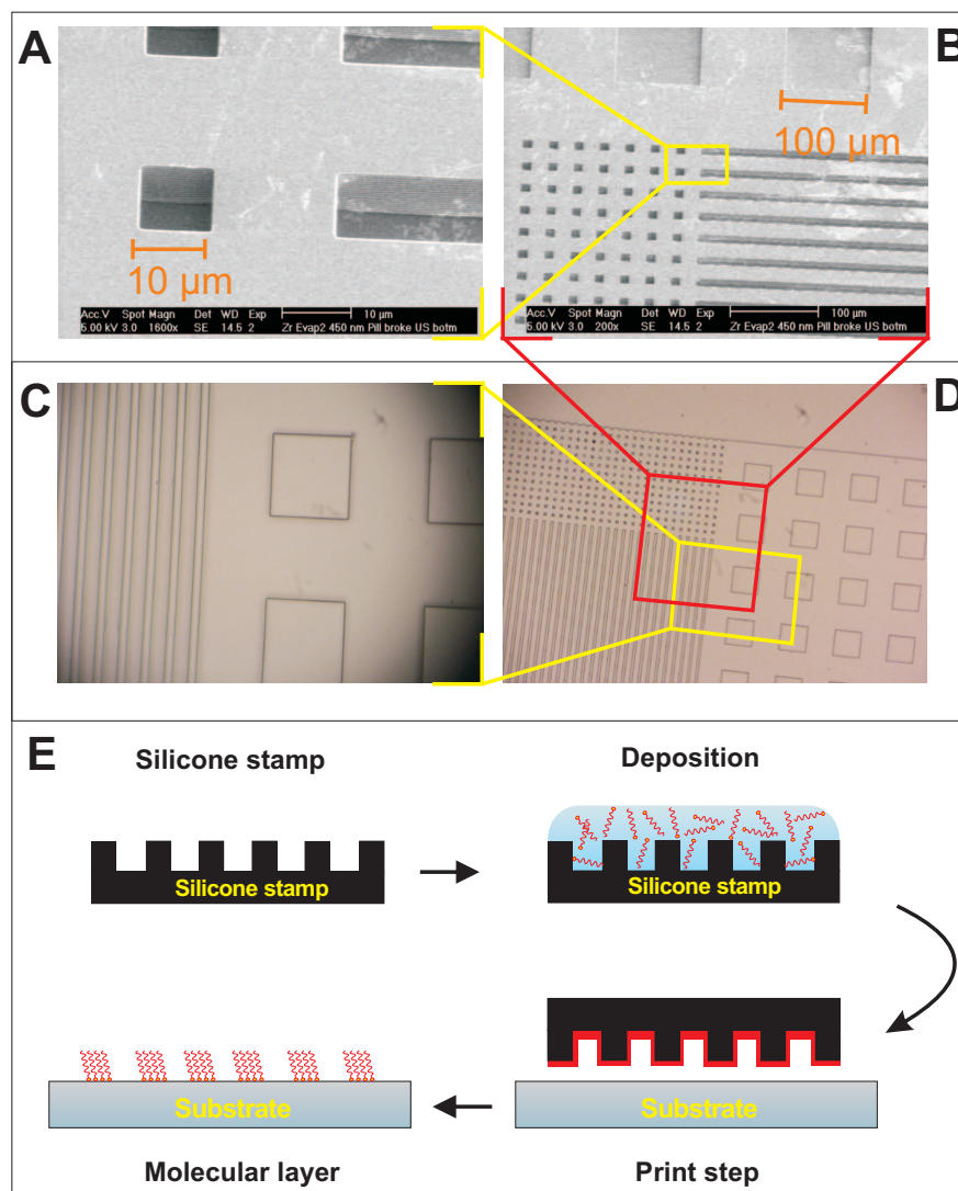
Figure 6.1: Representation of the different \mu cp steps involved in the realization of a molecular monolayer. A and B, SEM images of the silicon wafer; C and D, optical microscopy images of the used silicone stamp; E, molecular film production steps.
