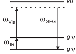
Figure 3.3: Energy level diagram of resonance/off-resonance SFG in the B-O approximation.
