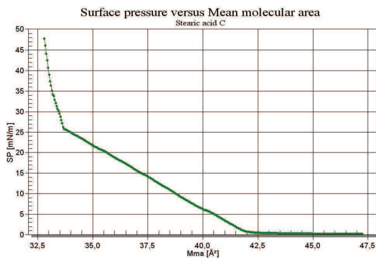
Figure 7.5: LB isotherm of stearic acid.
