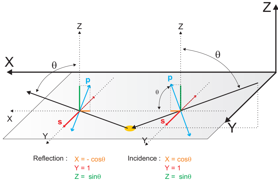
Figure 1.5: Projection of incident and reflected polarizations on xyz axes.
