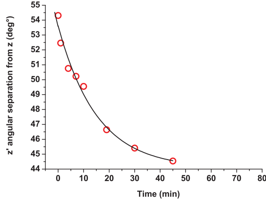
Figure 4.6: Evolution of the angular separation between the rhodamine z' axis and the surface normal z with time. The fluid viscosity is \eta = 20 mPa s and the flow speed is 20 cm/s. The decay constant \lambda is 6,57 \cdot 10^{-2} \text{ s}^{-1} , C = 44.1 , and A_0 = 9.55 .
