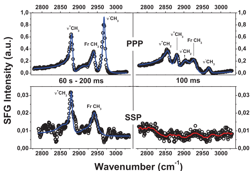
Figure 6.5: SFG spectra of printed HDT films recorded in ppp (upper panels) and ssp (lower panels) polarization for 60 s - 0,2 s (left) and 100 ms (right) printing durations. Below 200 ms, methyl vibrational activities are reduced by the methylene chain disorder.
