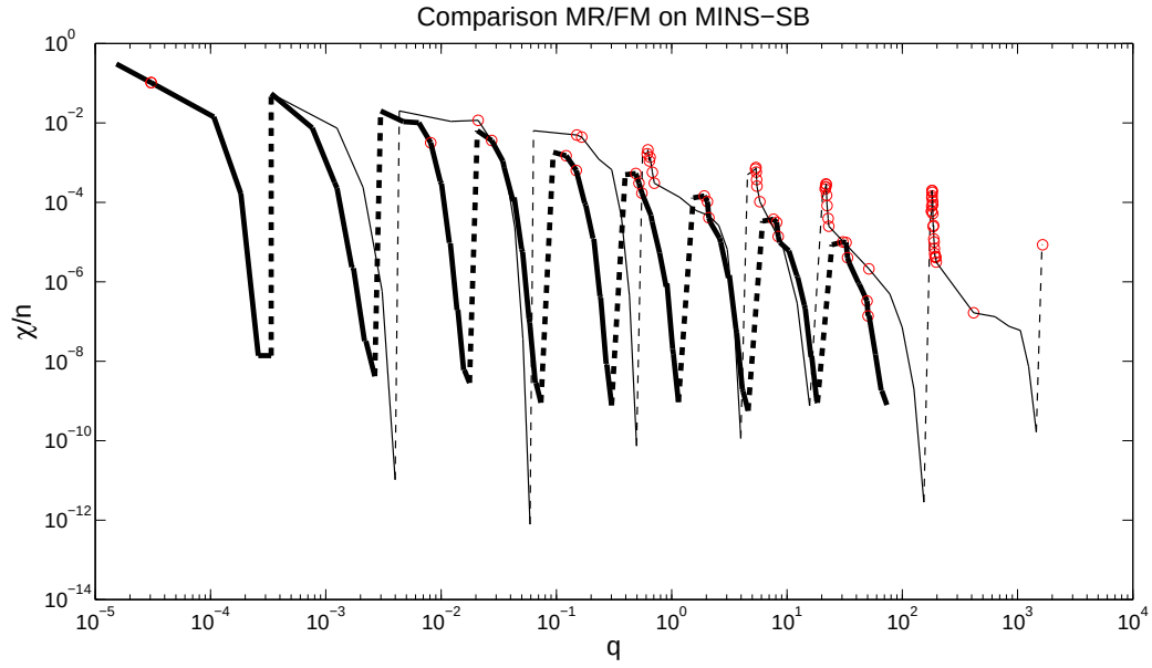
Figure 4.10: History of the scaled criticality measure on MINS-SB. A small circle surrounds the iterations where the trust region is active. As above, both axes are decadically logarithmic.
