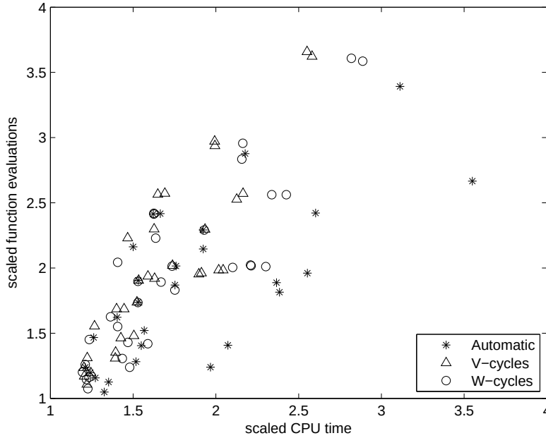
Figure 4.6: Average scaled function evaluations versus average scaled CPU-time for all algorithmic variants, distinguishing the type of recursive cycles.
