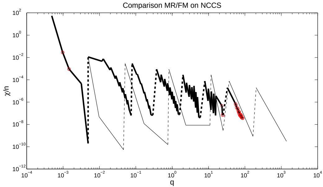
Figure 4.11: History of the scaled criticality measure on NCCS. A small circle surrounds the iterations trust region is active. As above, both axes are decadically logarithmic.
