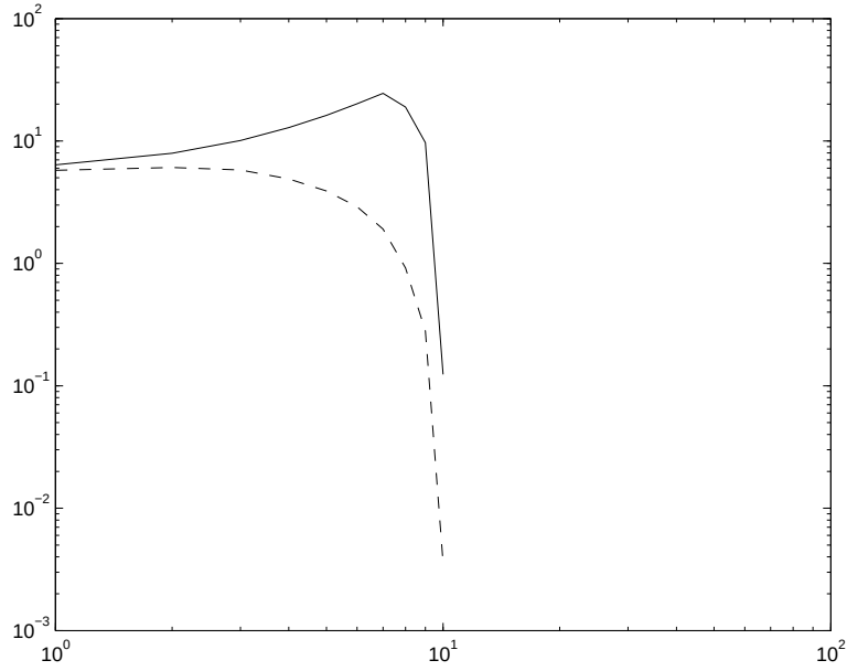
Figure 4.16: History of the two scaled criticality measures \chi^{tr}/n^r (plain line) and \chi^{out,1}/n^r (dashed line) on ACA-BC. As above, both axes are decadically logarithmic.
