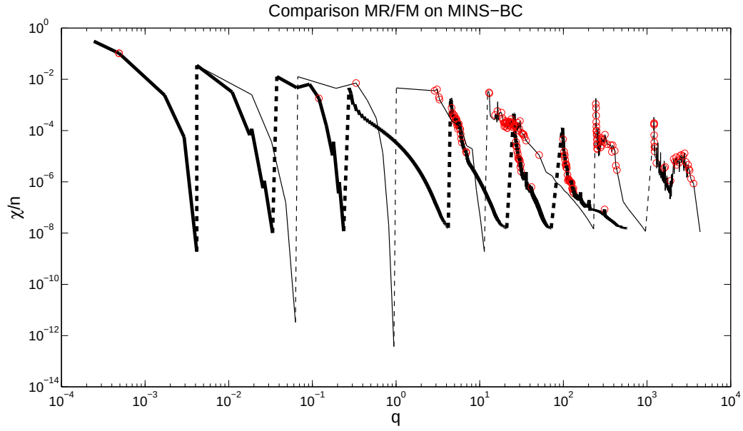
Figure 4.13: History of the scaled criticality measure on MINS-BC. A small circle surrounds the iterations where the trust region is active. As above, both axes are decadically logarithmic.
