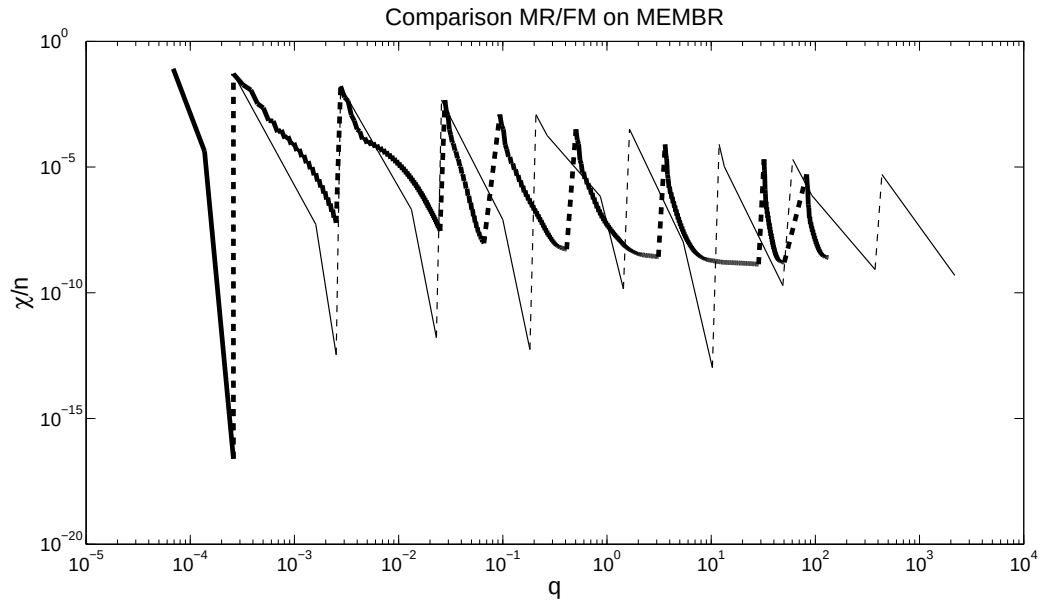
Figure 4.14: History of the scaled criticality measure on MEMBR. As above, both axes are decadically logarithmic.
