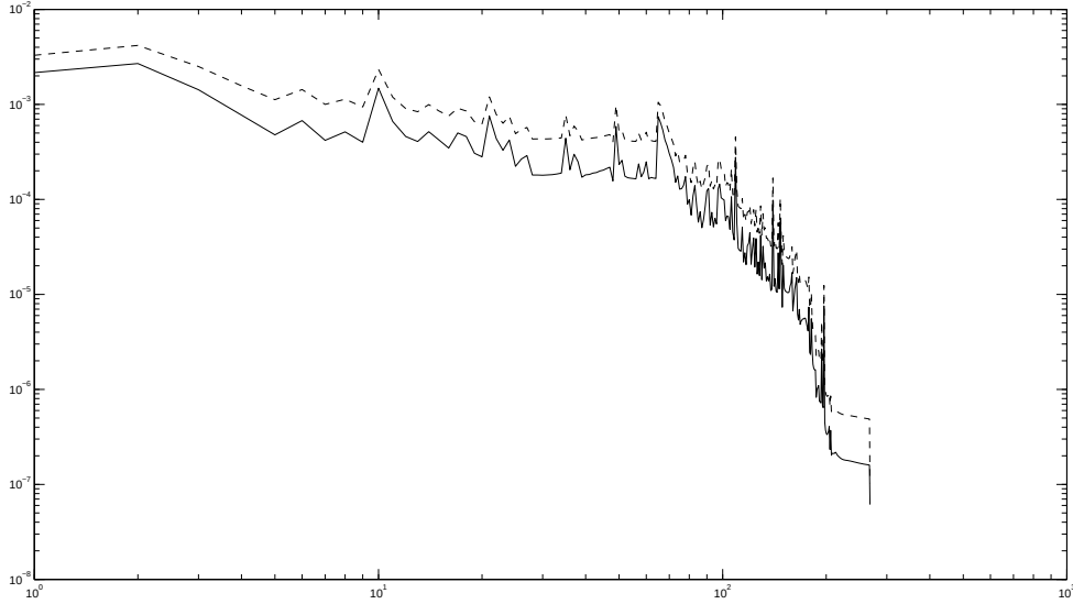
Figure 4.15: History of the two scaled criticality measures \chi^{tr}/n^r (plain line) and \chi^{out,1}/n^r (dashed line) on MINS-BC. As above, both axes are decadicly logarithmic.
