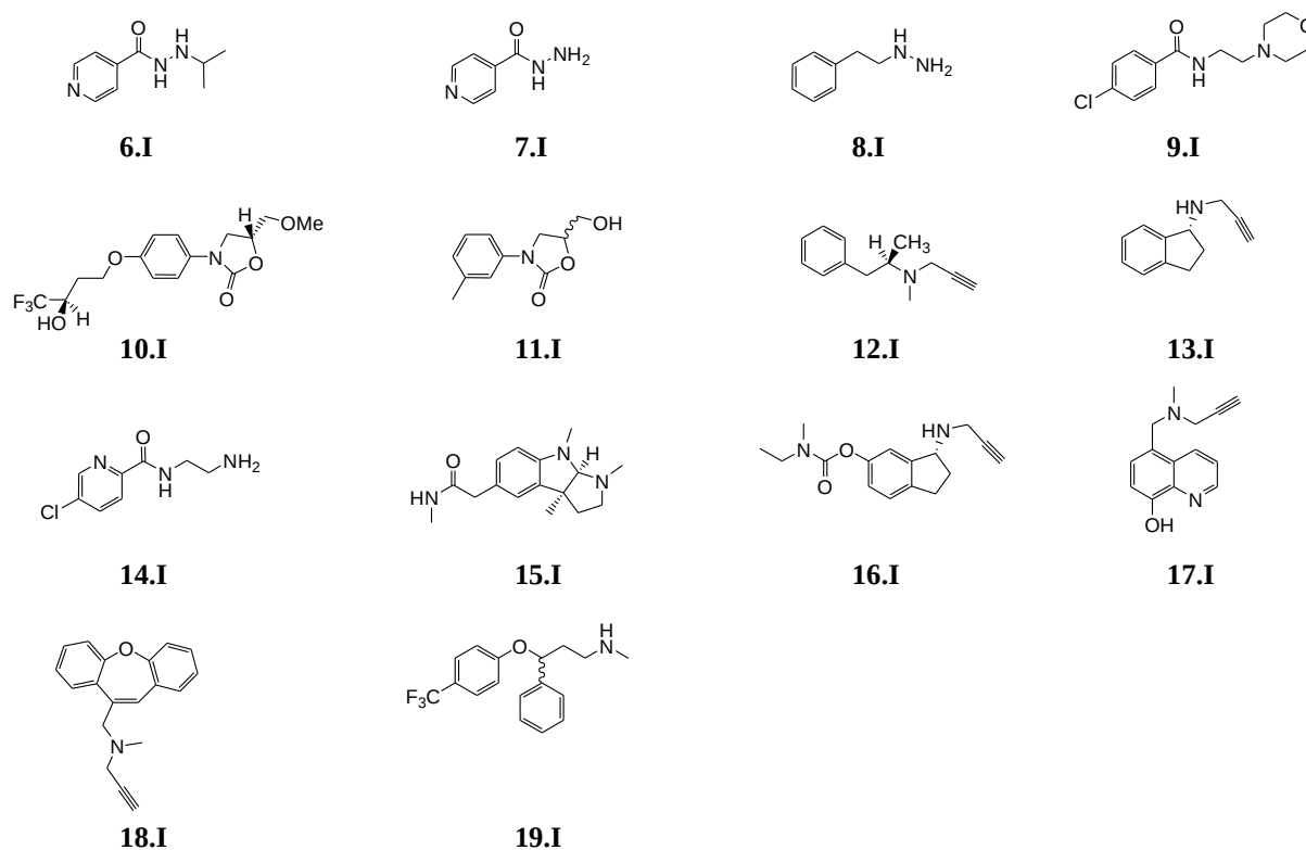
Figure 5.I. Chemical structures of iproniazid ( 6.I ), isoniazid ( 7.I ), phenelzine ( 8.I ), moclobemide ( 9.I ), befloxtatone ( 10.I ), tolloxatone ( 11.I ), l -deprenyl ( 12.I ), rasagiline ( 13.I ), lazabemide ( 14.I ), physostigmine ( 15.I ), ladostigil ( 16.I ), M30 ( 17.I ), CGP 3466 ( 18.I ) and fluoxetine ( 19.I ).
