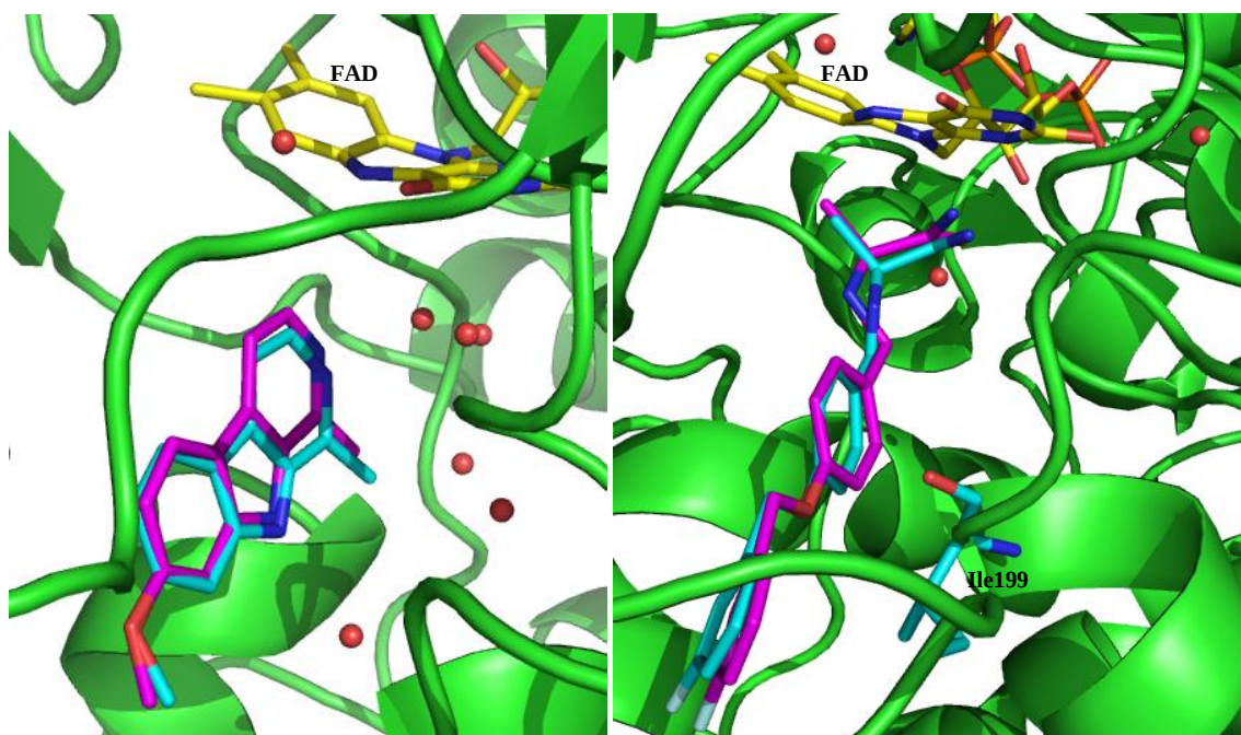
Figure 15.III. Superimposition of, (left) the crystal structure of hMAO-A (2Z5X.pdb) in complex with harmine ( 3.I , cyan) and the top docking solution of harmine in hMAO-A model (magenta), and (right) the crystal structure of hMAO-B (2V5Z.pdb) in complex with safinamide ( 1.I , cyan) and the top docking solution of safinamide in hMAO-B model (magenta). The water molecules are displayed as red spheres.
