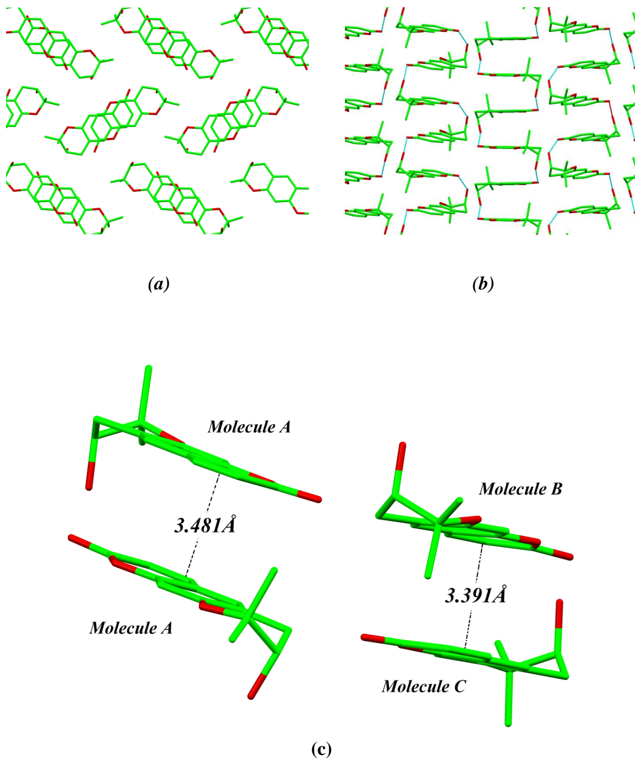
Figure 4.3.6. Crystal packing of aegelinol. (a) Stacking along the a axis; (b) Stacking along the b axis; (c) \pi - \pi stacking distances (Å) in aegelinol alone.
