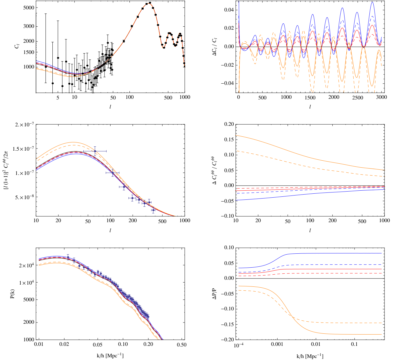
FIG. 1. CMB temperature angular power spectrum (top left), lensing potential power spectrum (middle left) and matter power spectrum (bottom left), as well as the corresponding relative difference between the K-mouflage and \Lambda CDM models (right panels), for the following parameter set combinations: K_0 = 100 , \beta = 0.2 (blue), K_0 = 100 , \beta = 0.1 (red), K_0 = -5 , \beta = 0.2 (orange), for m = 3 (solid lines) and m = 2 (dashed lines). The \Lambda CDM model used in the ratios is that with \Sigma m_\nu = 0 (solid black). In the upper left and middle left panels, the data points with errorbars correspond, respectively, to the CMB temperature and lensing potential power spectra as measured by the Planck satellite [30]. In the lower left panel, the data points show the SDSS-DR7 Luminous Red Galaxy (LRG) host halo power spectrum as presented in [31].
