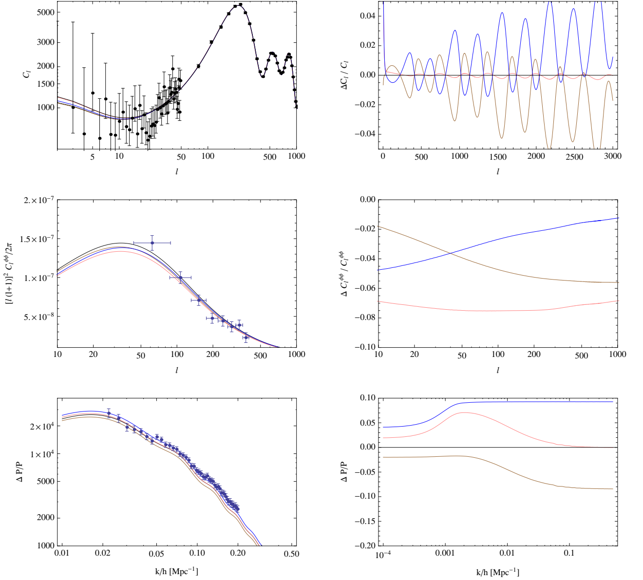
FIG. 3. CMB temperature angular power spectrum (top left), lensing potential power spectrum (middle left) and matter power spectrum (bottom left), as well as the corresponding relative difference between the K-mouflage and \Lambda CDM models (right panels), for K_0 = 50 , \beta = 0.2 , m = 3 and \Sigma m_\nu = 0.18 eV ( \Omega_\nu h^2 = 1.92 \times 10^{-3} , in pink). The \Lambda CDM model used in the ratios is that with \Sigma m_\nu = 0 (solid black). For comparison, the results for the LCDM model with massive neutrinos and \Omega_\nu h^2 = 1.92 \times 10^{-3} (brown) and for the K-mouflage model with same parameters and \Sigma m_\nu = 0 (blue) have been displayed. In the upper left and middle left panels, the data points with errorbars correspond, respectively, to the CMB temperature and lensing potential power spectra as measured by the Planck satellite [30]. In the lower left panel, the data points show the SDSS-DR7 Luminous Red Galaxy (LRG) host halo power spectrum as presented in [31].
