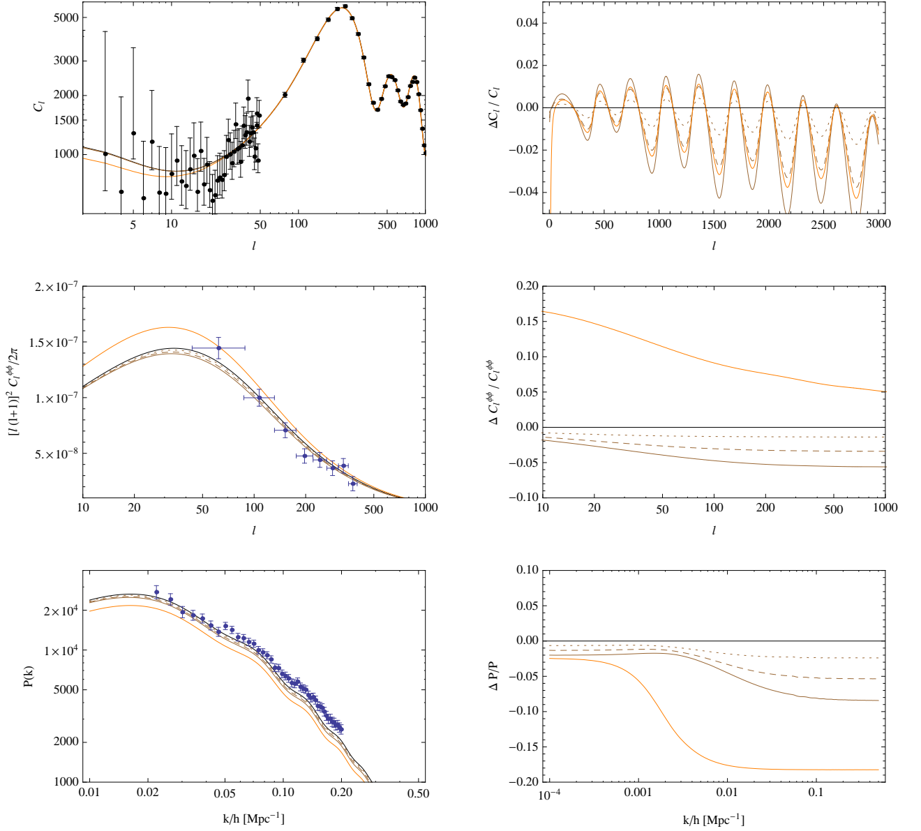
FIG. 2. CMB temperature angular power spectrum (top left), lensing potential power spectrum (middle left) and matter power spectrum (bottom left) for \Lambda CDM with \Omega_\nu h^2 = 0.64 \times 10^{-3} (dotted brown) corresponding to \sum_\nu m_\nu = 0.06 eV, \Omega_\nu h^2 = 1.28 \times 10^{-3} (dashed brown) corresponding to \sum_\nu m_\nu = 0.12 eV and \Omega_\nu h^2 = 1.92 \times 10^{-3} (solid brown) corresponding to \sum_\nu m_\nu = 0.18 eV. We consider three active neutrinos with a degenerate mass spectrum. The results for the K-mouflage model with K_0 = -5 , \beta = 0.2 , m = 3 are also displayed for comparison (solid orange line). The right panels show the corresponding relative differences to \Lambda CDM with \sum m_\nu = 0 (solid black). In the upper left and middle left panels, the data points with errorbars correspond, respectively, to the CMB temperature and lensing potential power spectra as measured by the Planck satellite [30]. In the lower left panel, the data points show the SDSS-DR7 Luminous Red Galaxy (LRG) host halo power spectrum as presented in [31].
