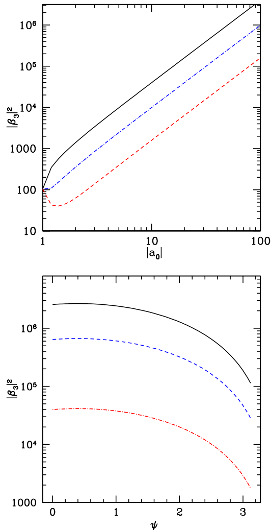
FIG. 2: In the top panel we show |\beta_3|^2 as a function of \alpha_0 for \alpha_0 and \beta_0 in phase (top, solid, black line), of opposite phase (lowest, dashed, red line) and with a phase difference of 0.8\pi (middle, dot-dashed, blue line).
