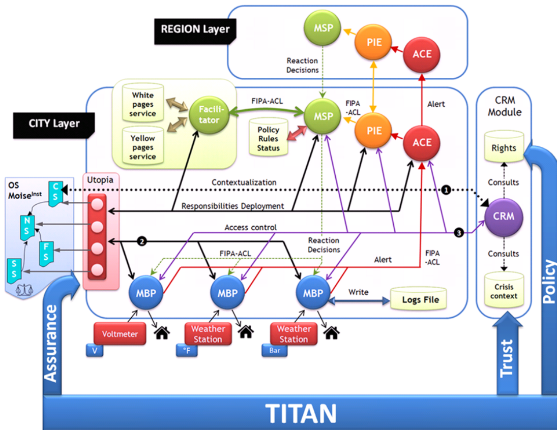
Figure 6 Detailed reaction architecture for power distribution adaptation based on weather parameters.
