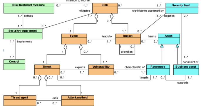
Fig. 1. ISSRM domain model (extracted from [5])
