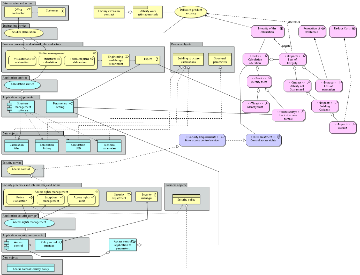
Fig. 5. @rchimed Extended Enterprise Architecture Model
