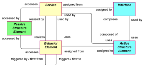
Fig. 2. ArchiMate modeling pattern (extracted from [4])
