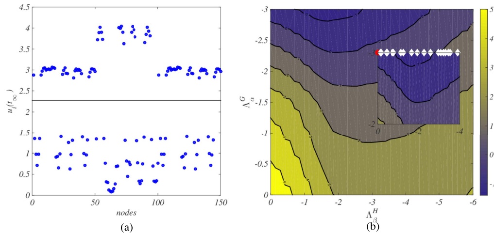
Figure 4. Turing patterns for the Mimura-Murray model on a degenerate multiplex support. The multiplex is built as the Cartesian product G \square H . Here, G = \bullet - \bullet - \bullet (namely, it is a linear chain with nearest neighbors connections) and H is a Watts-Strogatz 23 network composed by n_H = 50 nodes, with a probability to rewire a link equal to p_H = 0.04 and average degree \langle k_H \rangle = 4 . Panel (a): asymptotic distribution for the concentration of species u (circles, blue online) on each node of the Cartesian product G \square H . The recorded concentration varies from node to node and differs from the deputed equilibrium value \hat{u} \sim 2.28 (horizontal black line). For the selected parameters (see below), the Mimura-Murray model is Turing unstable on the linear chain G . Turing patterns cannot develop instead, when the reaction-diffusion model is made to evolve on the Watts–Strogatz network H alone. Panel (b): level sets of the function Q_{\alpha\beta}^{G \square H} . In the top border of the picture (region enlarged in the inset, dark blue online) the function assumes negative values. The (red online) circle identifies the unstable eigenvalue of the Laplacian operator associated to the linear chain. As anticipated, it falls in the region Q_{\alpha\beta}^{G \square H}(\Lambda_\alpha^G, 0) = Q^G(\Lambda_\alpha^G) < 0 , hence signaling the presence of Turing-like patterns on G . The white diamonds refer to the pairs (\Lambda_\alpha^G, \Lambda_\beta^H) for which Q_{\alpha\beta}^{G \square H}(\Lambda_\alpha^G, \Lambda_\beta^H) < 0 , thus implying the existence of the instability on the Cartesian product G \square H . We remark that for \Lambda_\alpha^G = 0 , the function Q_{\alpha\beta}^{G \square H} is positive definite: patterns cannot emerge when the diffusion of the interacting species is confined on graph H . Here, the diffusion coefficients are set to the representative values D_u^G = 0.005 , D_v^G = 1.8 , D_u^H = 0.12 and D_v^H = 1.3 . The initial condition is assigned as explained in the caption of Fig. 2.
