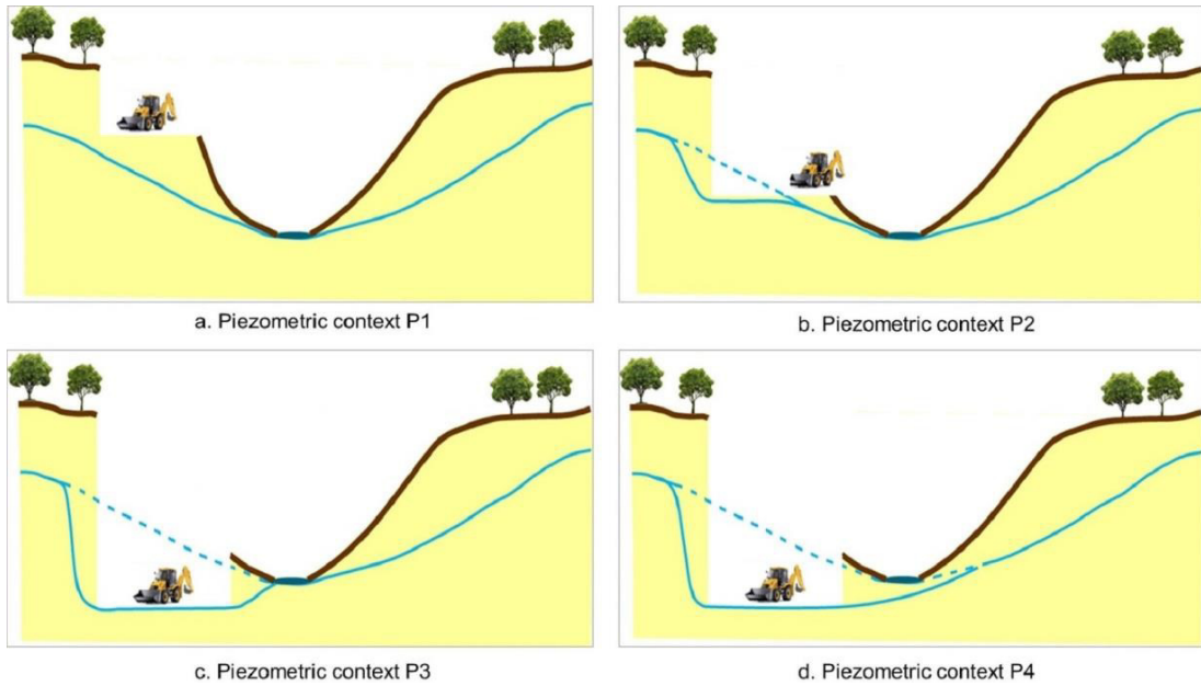
Fig.2. Maps illustrating the different piezometric settings.
