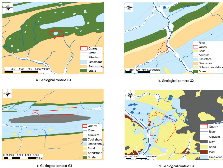
Fig.1. Maps illustrating the different geological settings.
