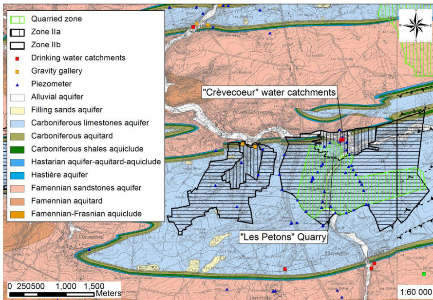
Fig.3. Map illustrating the exploitation of a quarry inside the zones IIa and IIb.
