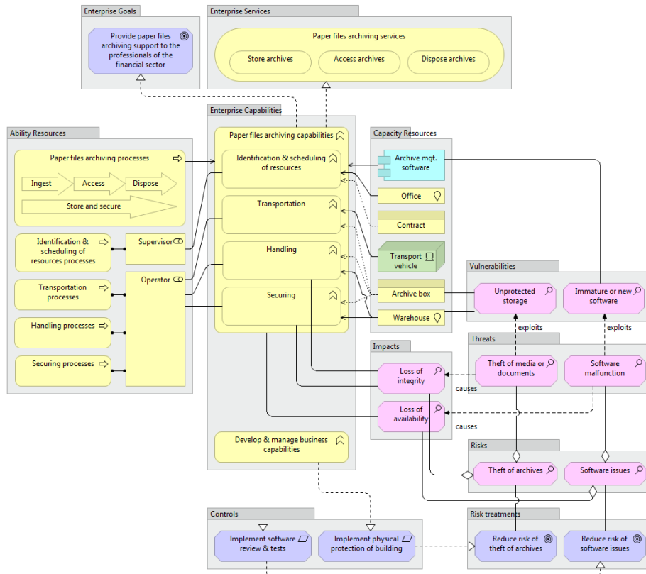
Fig. 4. Use case: Paper files archiving services
