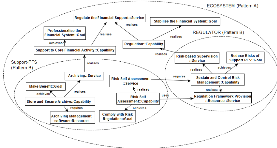
Fig. 3. Business Service Ecosystem metamodel instantiated to the financial system
