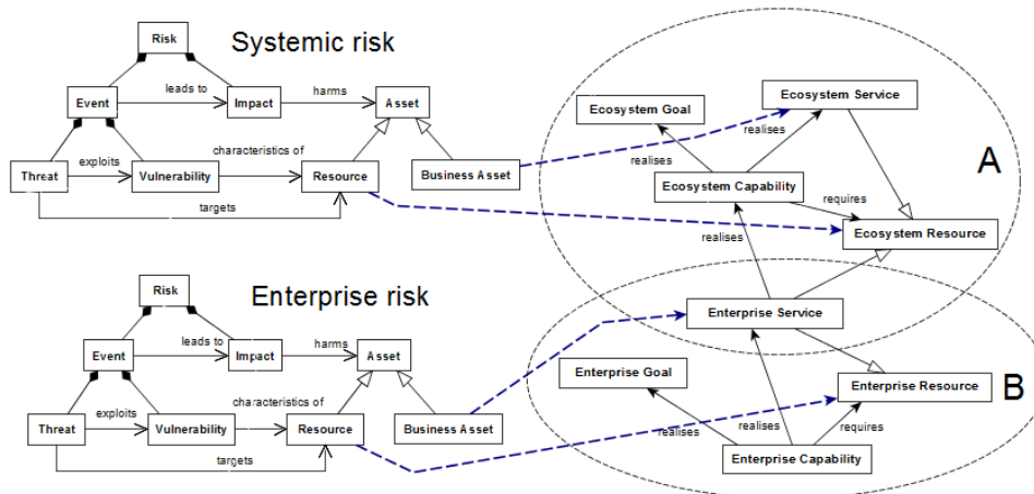
Fig.2. Mapping ISSRM – BSE metamodel
