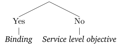
(b) The decision tree for the one-to-many relationship implying the Quality constraint class
