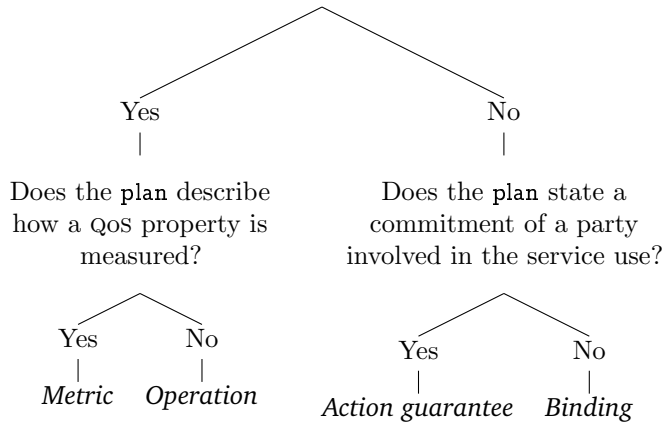
(c) The decision tree for the one-to-many relationship implying the Plan class
