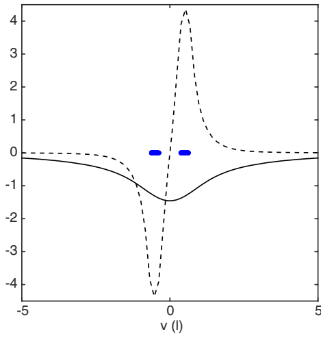
FIG. 8. (\rho(0, v) - \lambda(0, v))/C_I (straight line) and magnetic field B_z(0, v)/(\mu_0 N I) (dashed line) along the axis of symmetry of the anti-Helmholtz coil ( \mu_0 N I = 4.4T ). Dots indicate the position of the solenoids along the z axis.
