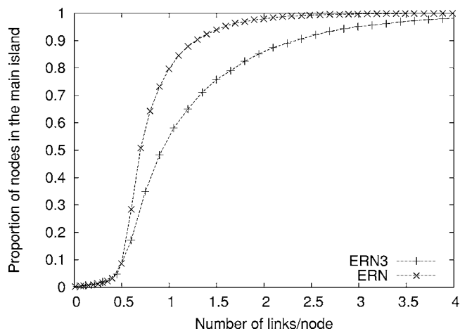
FIG. 9. Proportion of nodes in the main island, as a function of the number of links/node, in the ERN and the ERN (3) model. The networks are composed of 1000 nodes.
