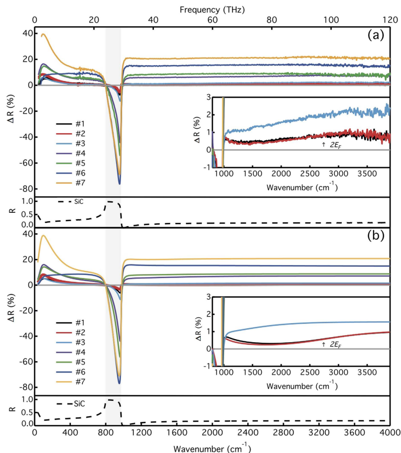
Figure 8. Differential reflectance spectra of the studied samples, together with SiC reflectance.
