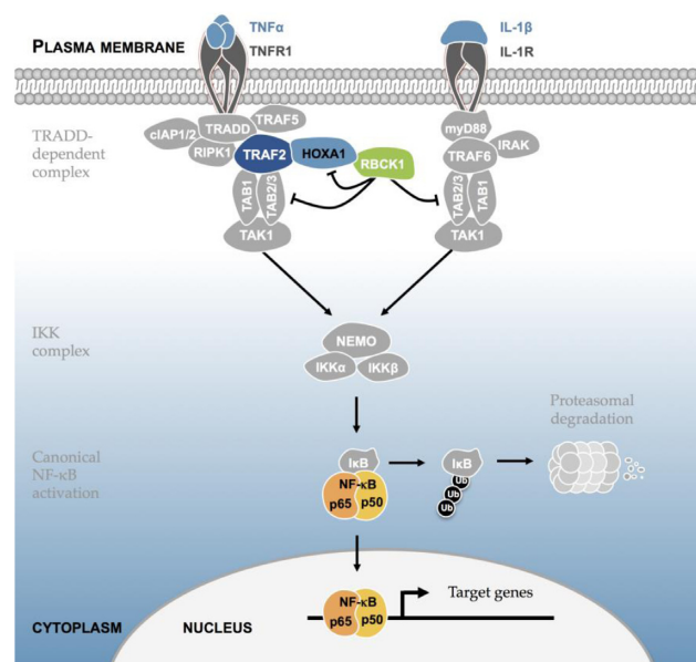
Figure 9. Model for the HOXA1-mediated modulation of the NF- \kappa B pathway. Upon TNF stimulation, TNF \alpha binding to TNFR initiates the recruitment of TRADD that further recruits cIAP1/2, RIPK1, TRAF2 and TRAF5 to form the TRADD-dependent complex. This leads to the docking of TAK1 in complex with TAB2 and TAB3, allowing formation of the IKK complex. The IKK complex phosphorylates I \kappa B, promoting its proteasomal degradation, allowing NF- \kappa B release and finally its nuclear translocation to engage transcriptional programs. On the one hand, HOXA1 enhances TRAF2 activity or stabilizes the TRADD-dependent complex to activate the TNF/NF- \kappa B pathway. On the other hand, RBCK1 inhibits HOXA1 as well as TAB2/3 to repress NF- \kappa B activation. In addition, RBCK1 and TRAF2 can compete with each other to bind either the 11-His repeat or the homeodomain of HOXA1 (not represented).
