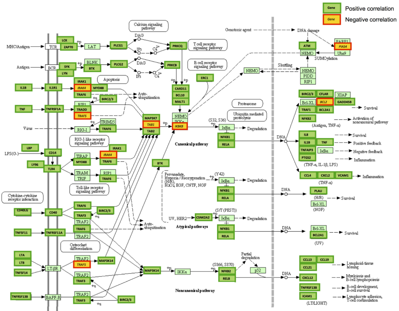
Figure 1. NF- \kappa B pathway genes with correlation to HOXA1 expression in breast cancer. Graphical overview of the NF- \kappa B pathway showing pathway genes with a significant correlation to HOXA1 expression in the Bertucci-266 dataset. The KEGG NF- \kappa B pathway graph with constituent genes (in pale green boxes with narrow border) is overlaid with boxes representing positively or negatively correlating genes (gene name on a green background with thick green border, or on a yellow background with thick red border, respectively). More details on correlations are in Table 1. The overview shows an almost comprehensive positive correlation with HOXA1 mRNA expression, strongly suggesting that the NF- \kappa B pathway is activated by HOXA1 in breast cancer cells.
