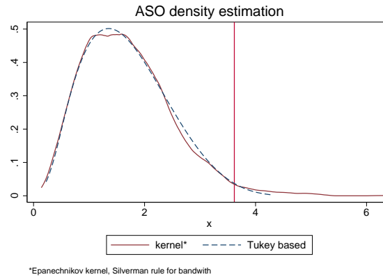
FIGURE 5. Kernel and Tukey-based estimations of the density of the asymmetrical outlyingness measures ASO_i for the data of the CDC ( n = 3143 , p = 3 )
