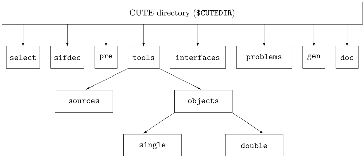
Figure 1: Organization of the CUTE directories
