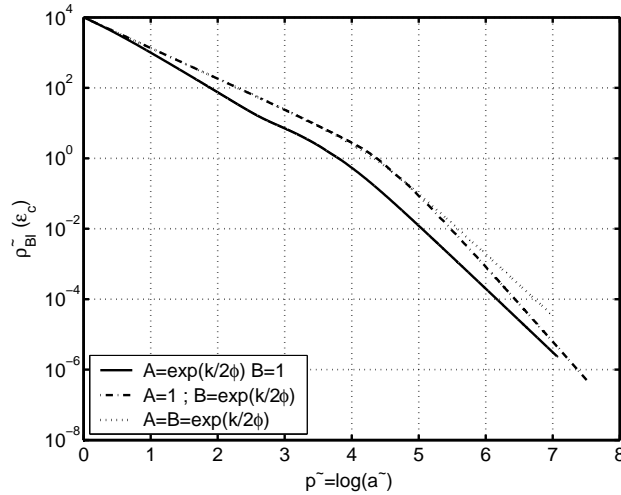
Fig. 8: Evolution of the physical energy density \tilde{\rho} with \tilde{p} = \ln(\exp(k/2\phi)a) for the curves in Figure 7 (Same parameters as above)
