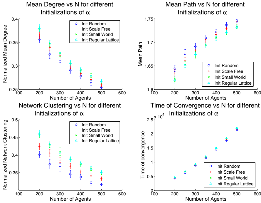
Fig. 8 Evolution the main network measures at the convergence of the opinions as its size (N) change, for different initial topologies. All the trends are referred to sets of 10 simulations with \sigma=0.5 , \alpha_c=0.5 and with \Delta O_c = 0.5 . The last image represent the average and the standard deviation of the time of convergence for the different topologies of the affinity matrix ( \alpha ) as they evolve with the size of the model.
