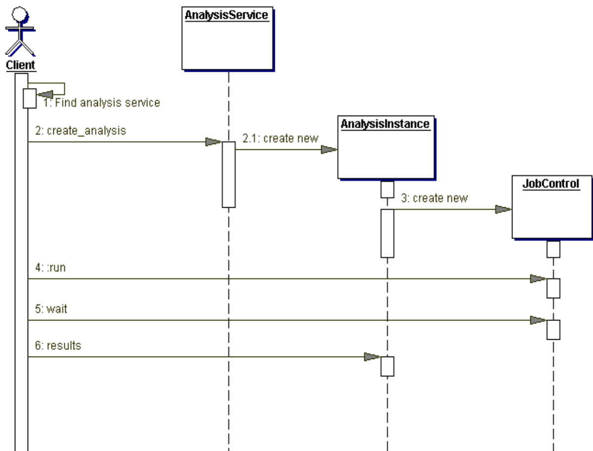
Figure 13 : Invocation synchrone
