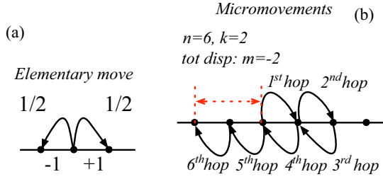
FIG. 1. The walker is allowed to perform at each step n elementary moves, each one having equal probability 1/2 to be in the positive or negative direction (a). In panel (b), we present a possible avalanche, where the walker performs n = 6 hops, two in the positive direction and 4 in the negative one, for a total effective displacement of m = -2 .
