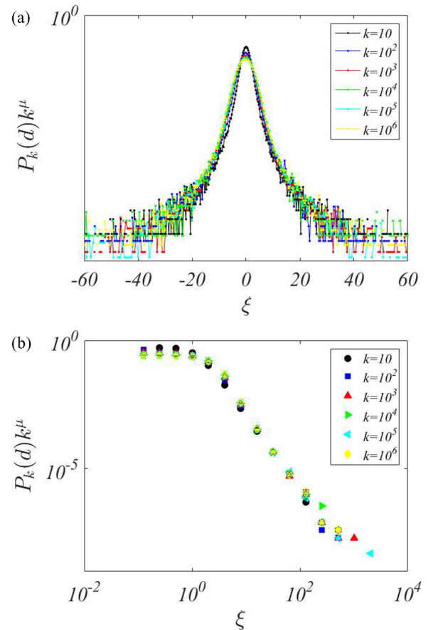
FIG. 3. Probability distribution P_k(d) in the discrete case for \gamma = 1.9 for N = 10^5 and a simulation time k = 10^6 with \mu = \frac{1}{2(\gamma-1)} and \xi = \frac{d}{k^{1/2(\gamma-1)}} . In (a) the curves superposition illustrates the self-similarity of the PDF and we display in (b) the power-law tail of the Lévy distribution. The color code in (a) and symbols in (b) refer to different k as specified in the legend.
