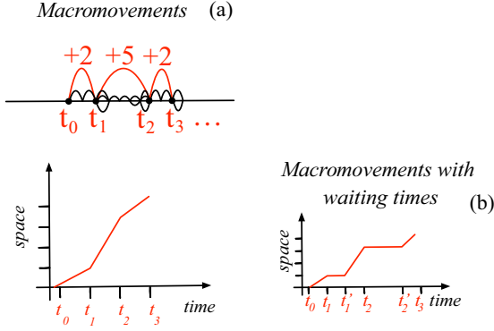
FIG. 2. In the continuous time frame, at each time t_i the walker can, as before, perform n microscopic moves: in panel (a) these macromovements result in displacements of m = 2 , m = 5 , and m = 2 . If we introduce the waiting times, the displacements are interspersed by waiting intervals: in panel (b) the walker stays put from t_1 to t'_1 and from t_2 to t'_2 .
