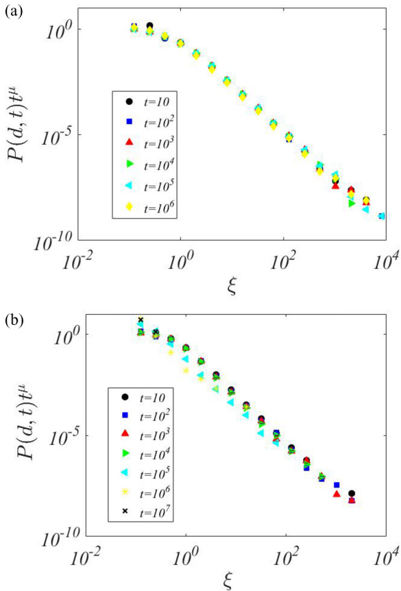
FIG. 4. Probability distribution P(d, t) in the continuous time case for (a) \alpha = 0.5, \gamma = 1.6 and (b) \alpha = 0.8, \gamma = 1.7 for N = 10^5 , where \mu = \frac{\alpha}{2(\gamma-1)} and \xi = \frac{d}{t^{\alpha/2(\gamma-1)}} . Again, the self-similarity of the PDF emerges once the curves are rescaled with respect to the \mu exponent.
