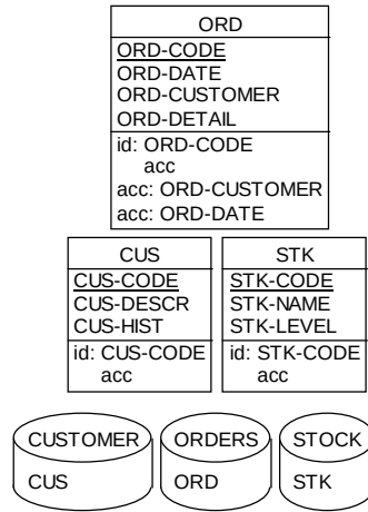
Figure 1.6: Example of DB-MAIN physical schema
