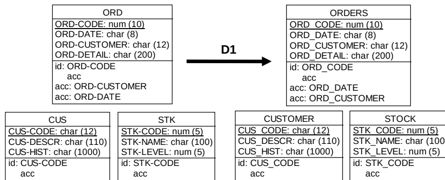
Figure 7.7: D1 conversion of the case study
