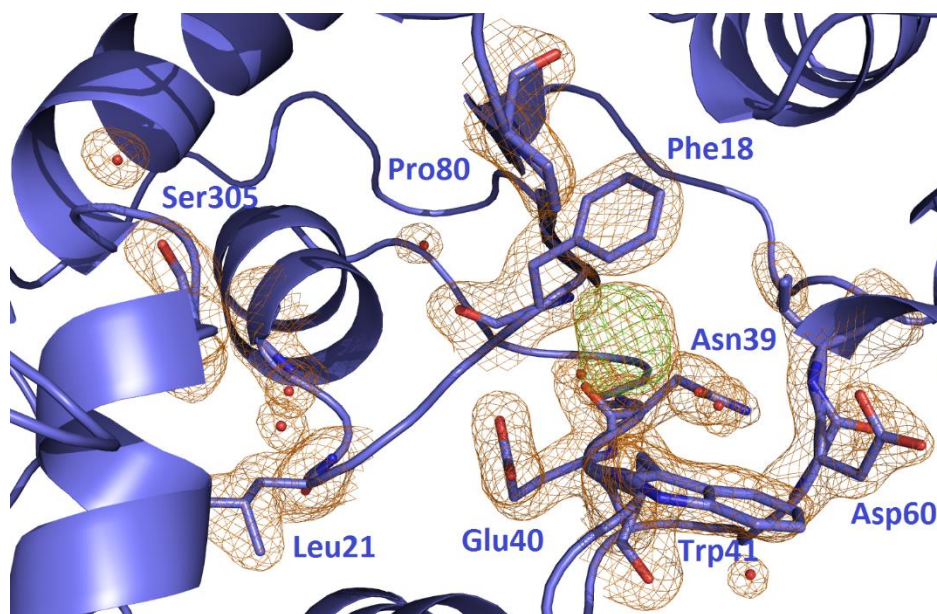
Figure 2. Structure of the M.HhaI apoenzyme. Solid Ribbon representation of cofactor binding site with 2Fo-Fc electron density map contoured at 1.0 \sigma for residues (orange mesh) normally involved in cofactor interaction and a Fo-Fc omit map contoured at 2.0 \sigma (green mesh) near the cofactor-binding site.
