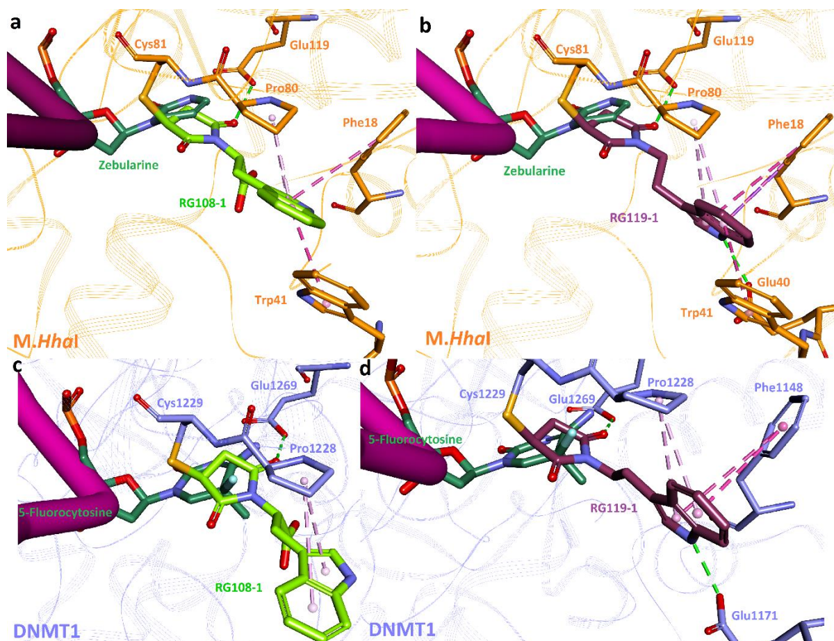
Figure 5. Covalent docking of RG108-1 and RG119-1 into bacterial M.HhaI and mouse DNMT1 .
