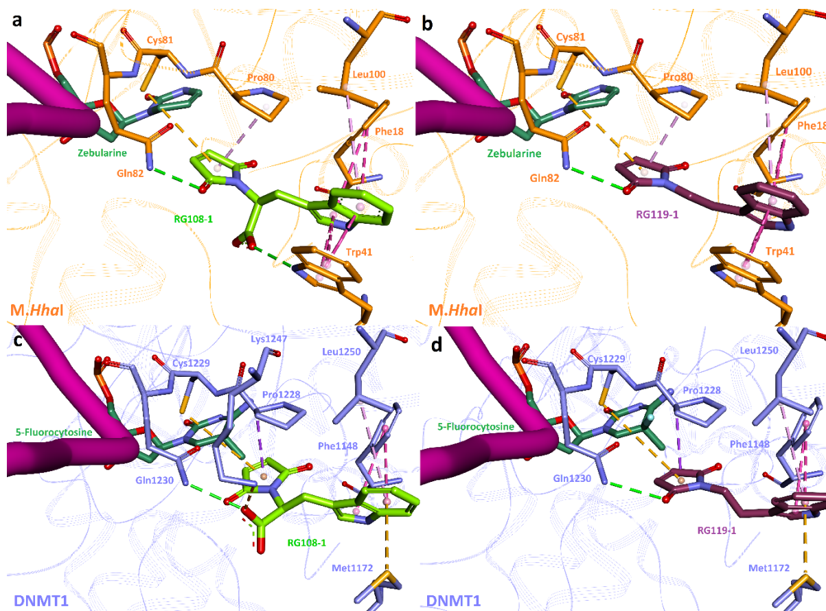
Figure 4. Non-covalent docking of RG108-1 (a,c) and RG119-1 (b,d) into bacterial M.HhaI (top) and mouse DNMT1 (bottom). Ligands and amino acid residues of the binding site are rendered as stick models while rest of the protein backbone is displayed as line ribbon. DNA backbone is displayed as purple tube model. Zebularine and 5-Fluorocytosine, removed prior to docking simulations, were added for final visualization. Molecular interactions are shown in dotted lines with the following color codes: green for conventional hydrogen bond, yellow for \pi -sulfur interaction, orange for salt bridge, purple for \pi -sigma interaction, light pink for \pi -alkyl interaction and pink for \pi - \pi stacking interaction. (a and b) Details of the binding mode of RG108-1 (a; green; docking pose) and RG119-1 (b; purple; docking pose) to M.HhaI (orange; PDB code: 1M0E). RG108-1 and RG119-1 both interact with M.HhaI via hydrogen bond involving Gln82, van der Waals interaction involving Pro80 and Leu100, \pi - \pi T-shaped interaction involving Phe18, parallel \pi - \pi stacking interaction involving Trp41 and \pi -sulfur interaction involving Cys81. RG108-1 makes an additional interaction with Trp41 by hydrogen bonding. (c and d) Details of the binding mode of RG108-1 (c; green; docking pose) and RG119-1 (d; purple; docking pose)
