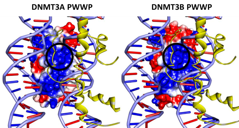
Figure 5. PWWP domains in complex with H3K36me3-NCP. PWWP domains surface colored by electrostatic potential of the residues (red: negatively charged area and blue: positively charged area). The black circle represents the zone of interaction between the aromatic cage of DNMT3s PWWP domains and the epigenetic mark H3K36me3.
