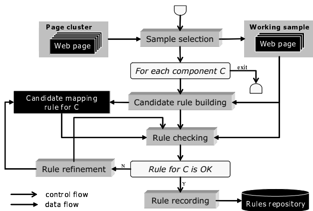
Figure 3. Mapping rules building scenario
